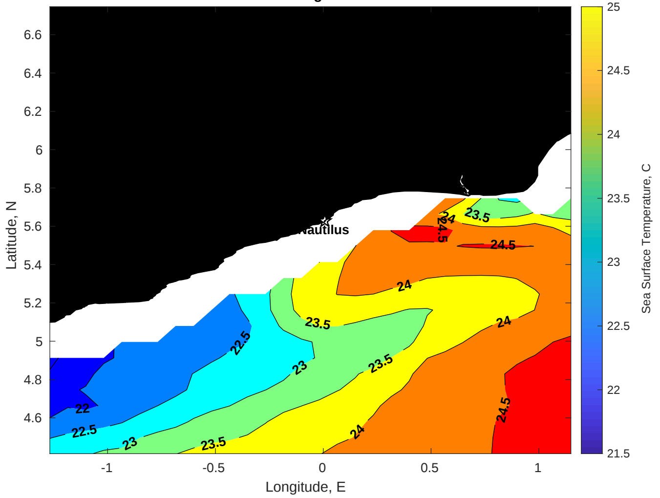
SST for Nautilus at 21-Aug-2025 00:00:00
