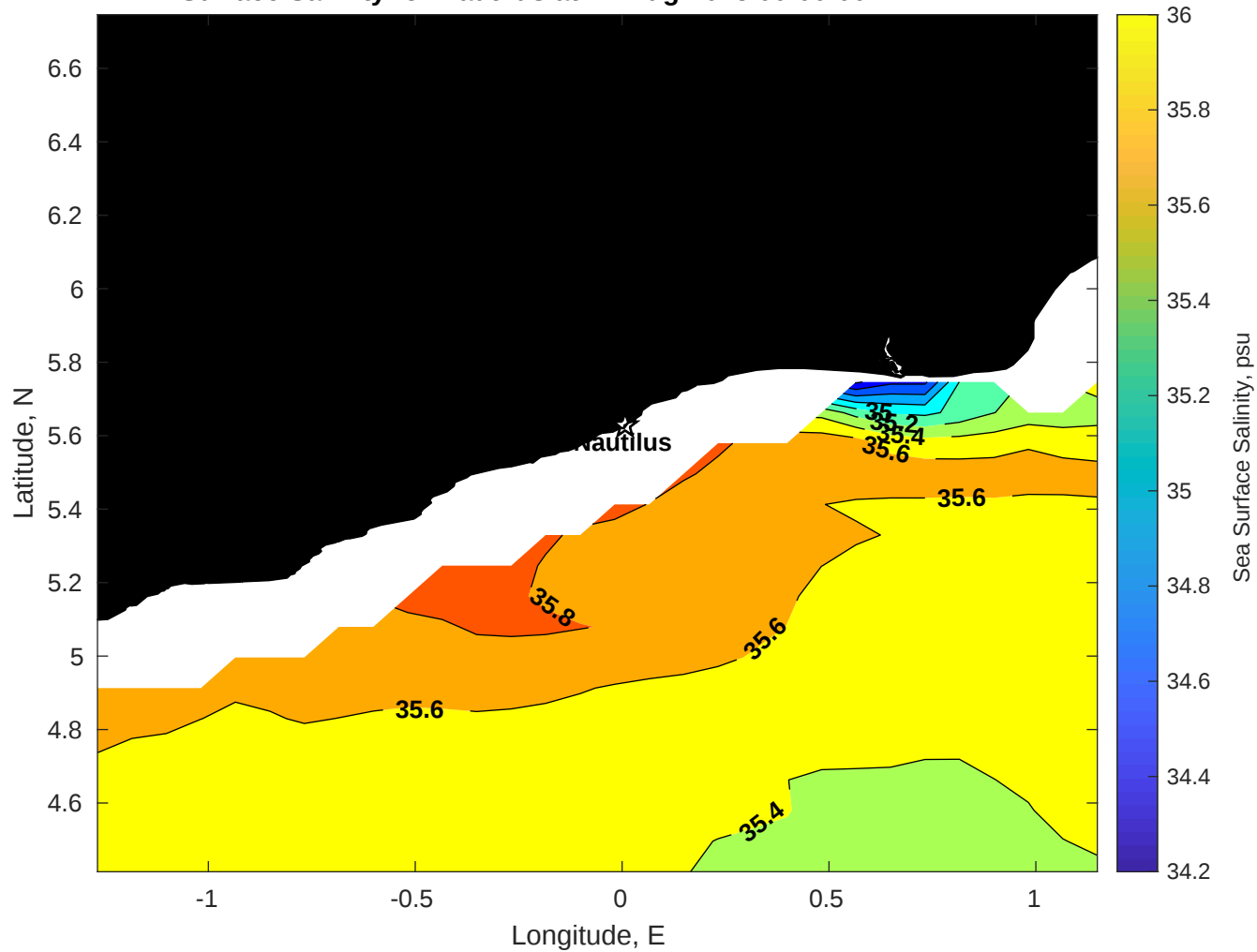
Surface Salinity for Nautilus at 21-Aug-2025 00:00:00
