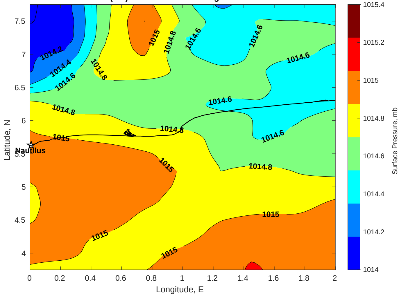
Surface Pressure (mb) for Nautilus at 22-Aug-2025 00:00:00
