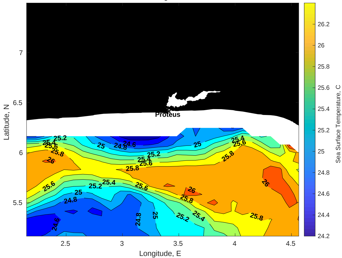
SST for Proteus at 21-Aug-2025 00:00:00
