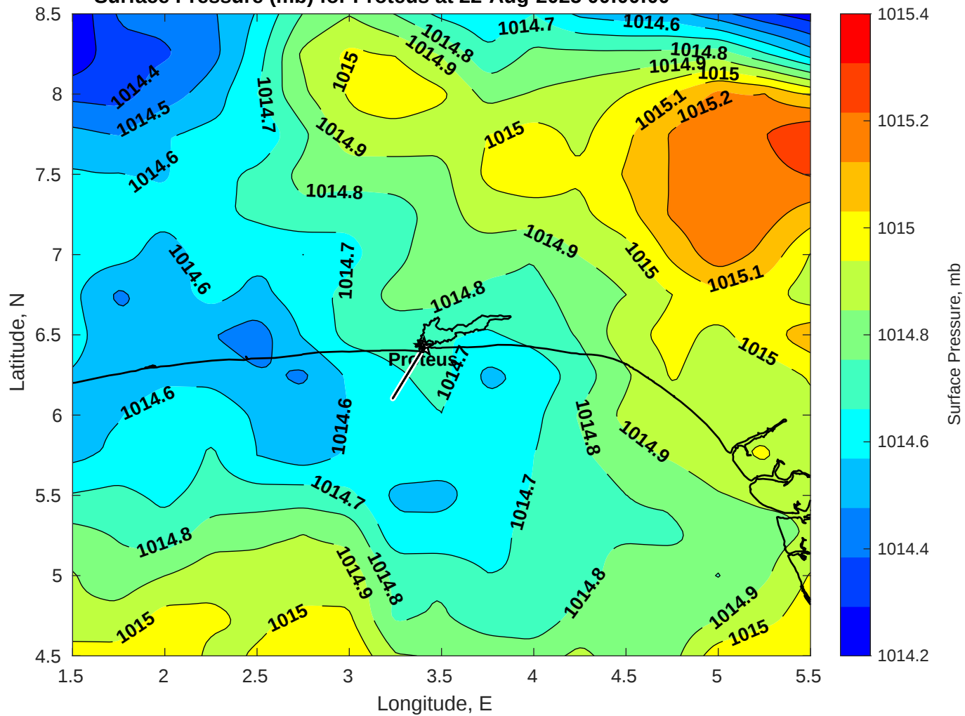
Surface Pressure (mb) for Proteus at 22-Aug-2025 00:00:00
