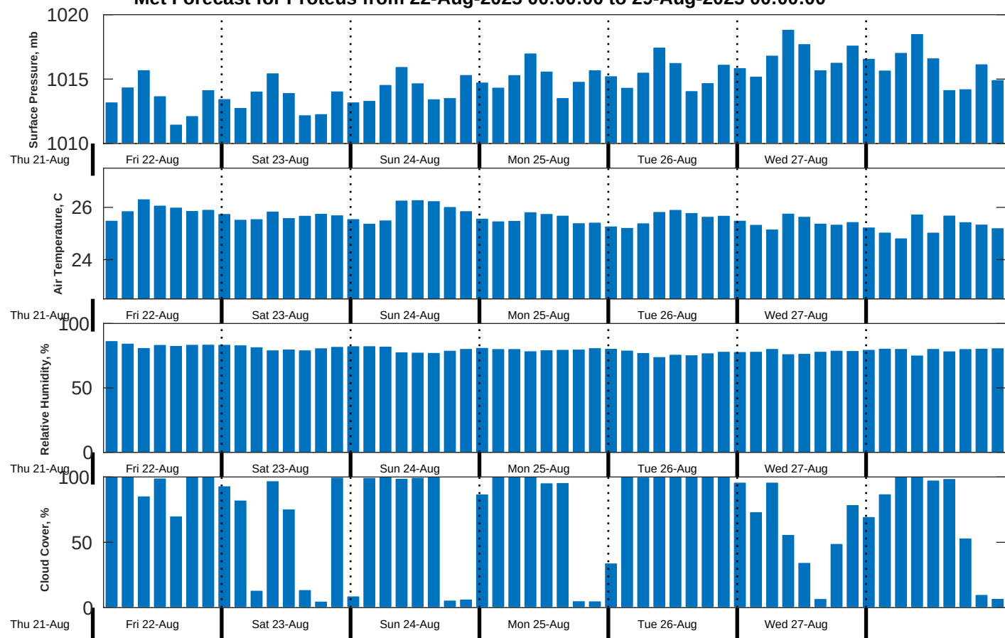
Met Forecast for Proteus from 22-Aug-2025 00:00:00 to 29-Aug-2025 00:00:00
