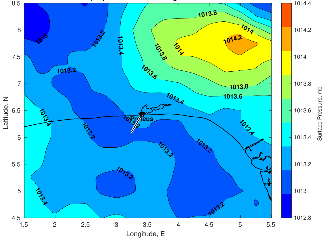
Surface Pressure (mb) for Proteus at 24-Aug-2025 00:00:00
