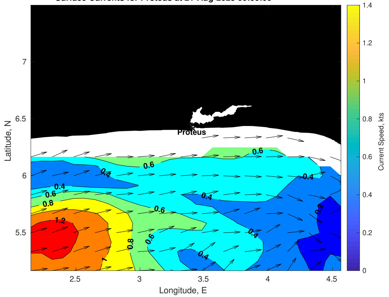
Surface Currents for Proteus at 21-Aug-2025 00:00:00
