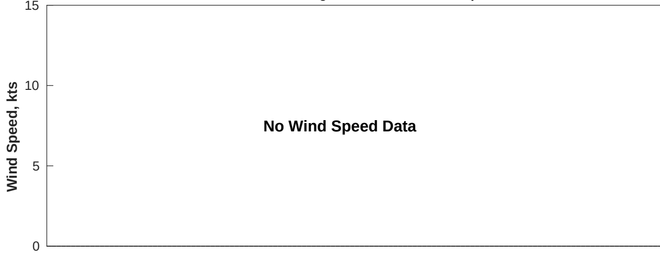
Wind & Wave Forecast for Proteus from 22-Aug-2025 01:00:00 to 07-Sep-2025 01:00:00
