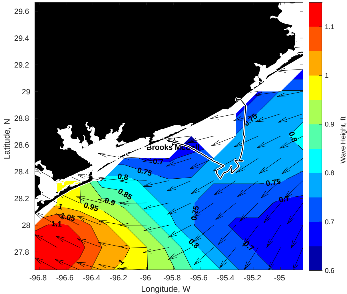
Wave Height (ft) for Brooks McCall at 23-Aug-2025 09:00:00
