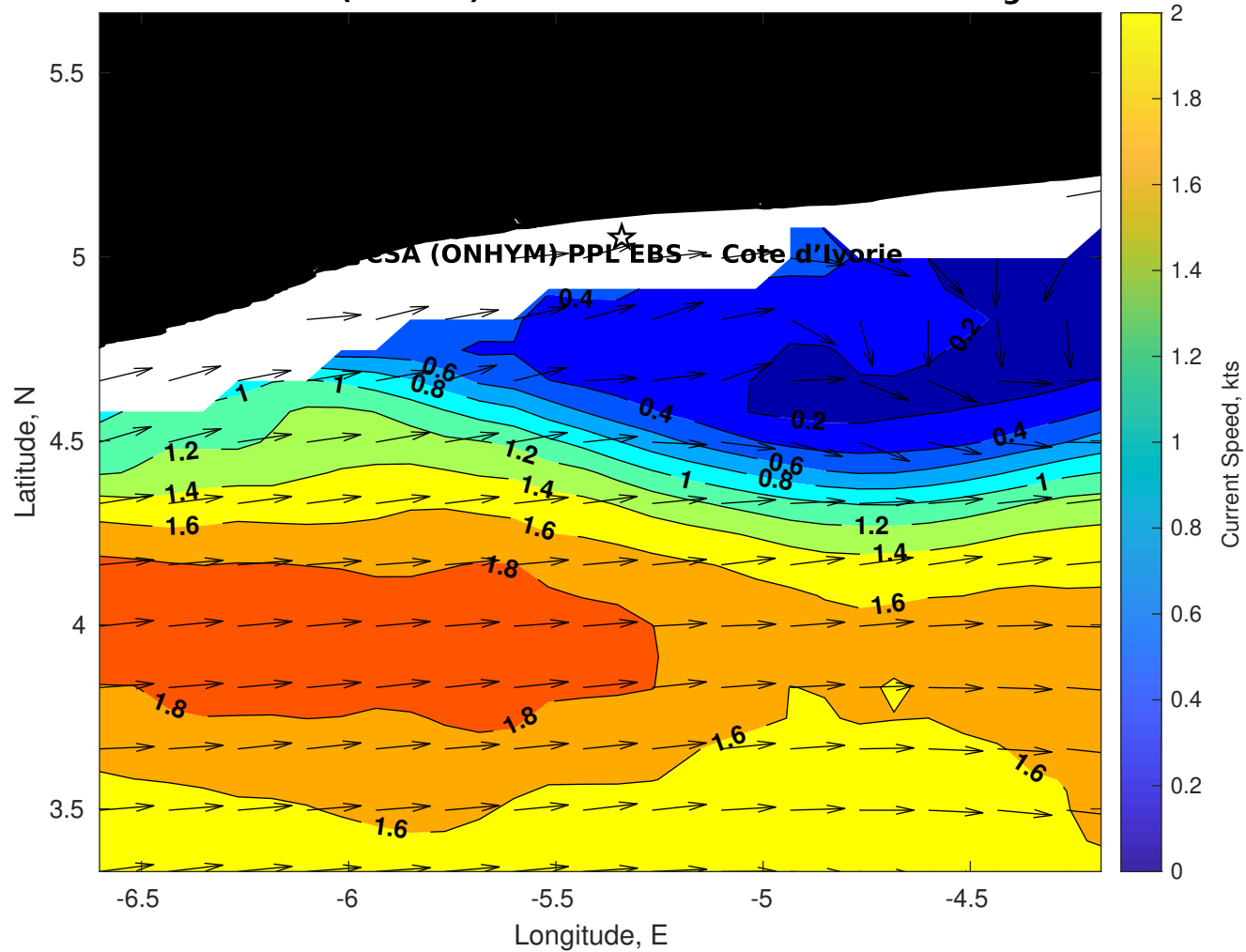
Surface Currents for CSA (ONHYM) PPL EBS - Cote d'Ivoire at 22-Aug-2025 00:00:00
