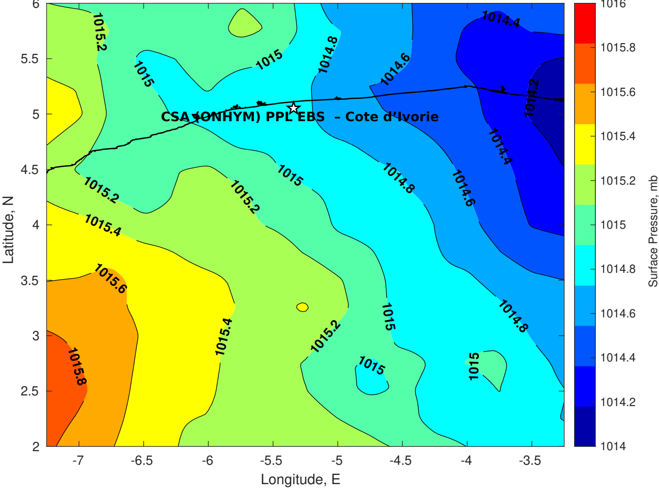
Surface Pressure (mb) for CSA (ONHYM) PPL EBS - Cote d'Ivoire at 23-Aug-2025 00:00:00
