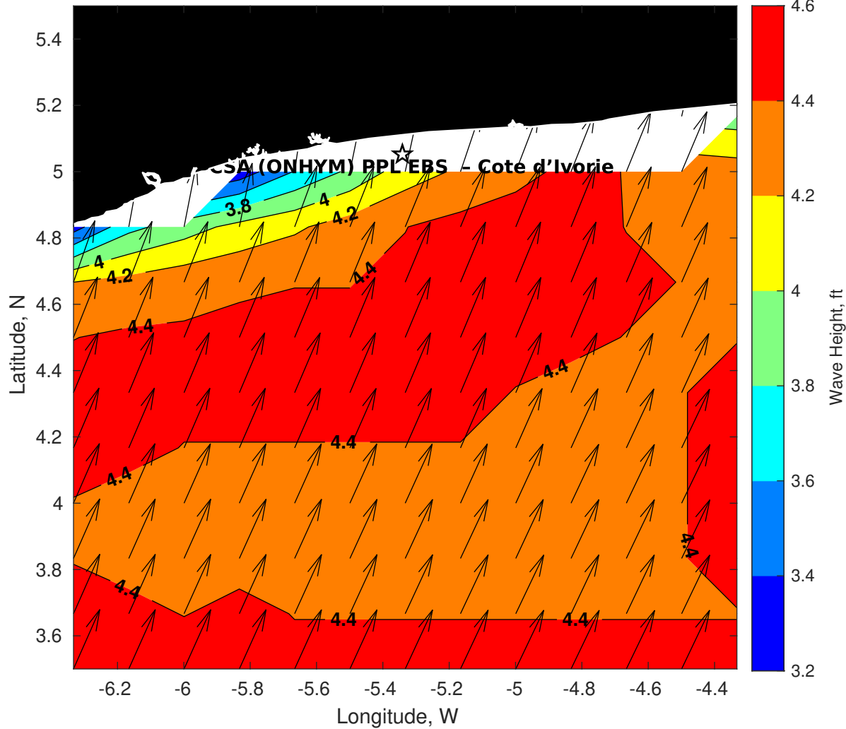
Wave Height (ft) for CSA (ONHYM) PPL EBS - Cote d'Ivoire at 23-Aug-2025 09:00:00
