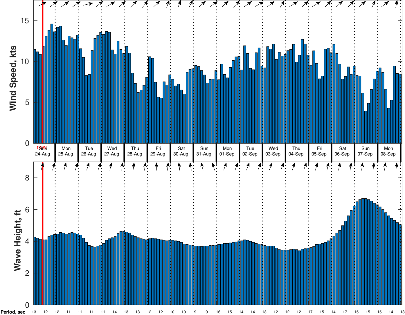
Wind & Wave Forecast for CSA (ONHYM) PPL EBS - Cote d'Ivoire from 23-Aug-2025 01:00:00 to 08-Sep-2025 01:00:00
