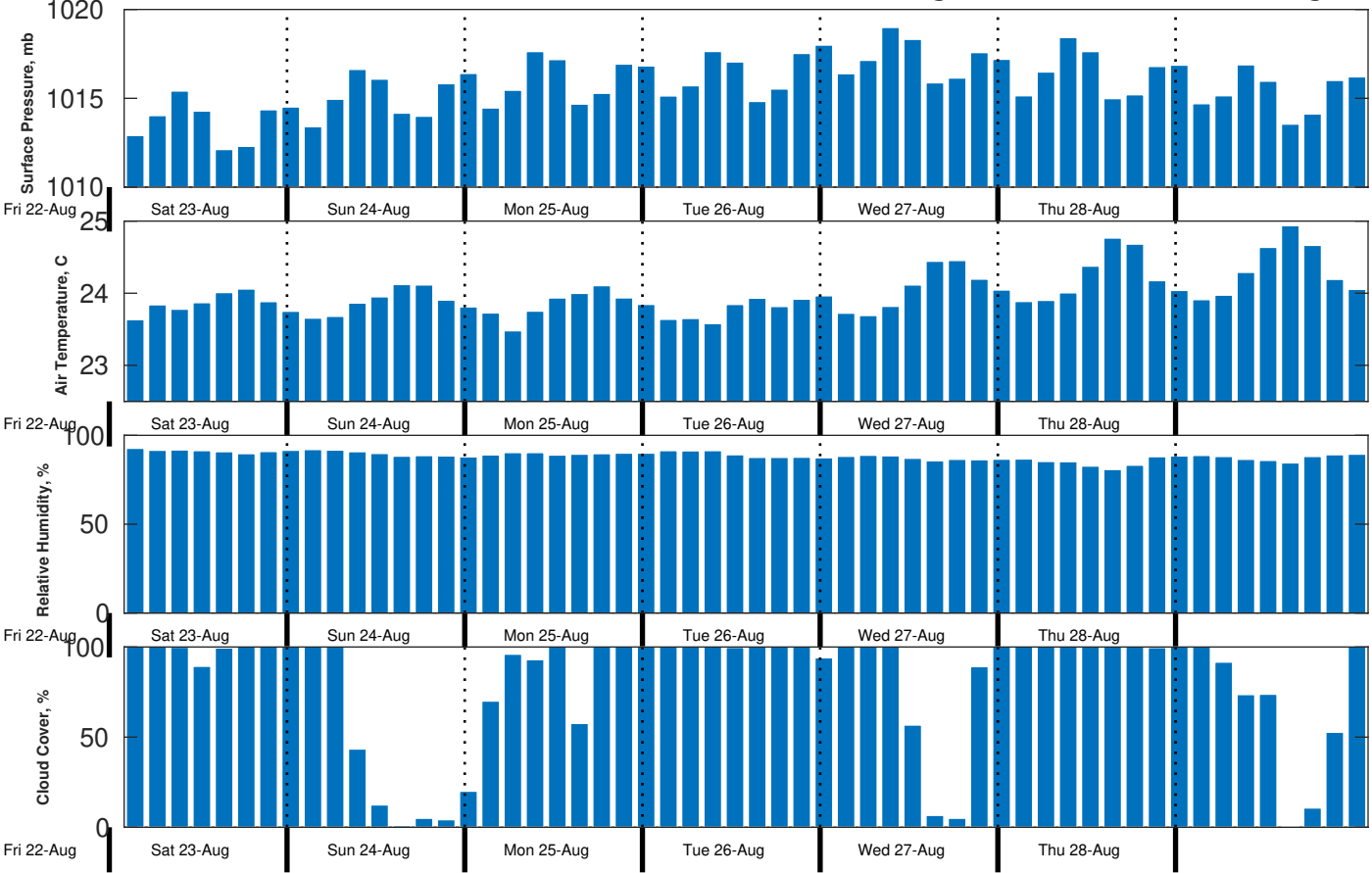
Met Forecast for CSA (ONHYM) PPL EBS - Cote d'Ivoire from 23-Aug-2025 00:00:00 to 30-Aug-2025 00:00:00
