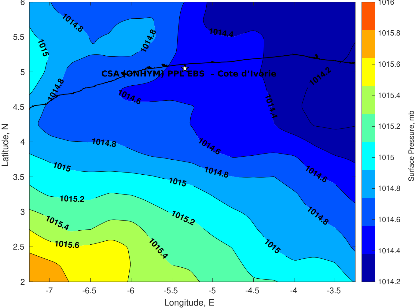
Surface Pressure (mb) for CSA (ONHYM) PPL EBS - Cote d'Ivoire at 24-Aug-2025 00:00:00
