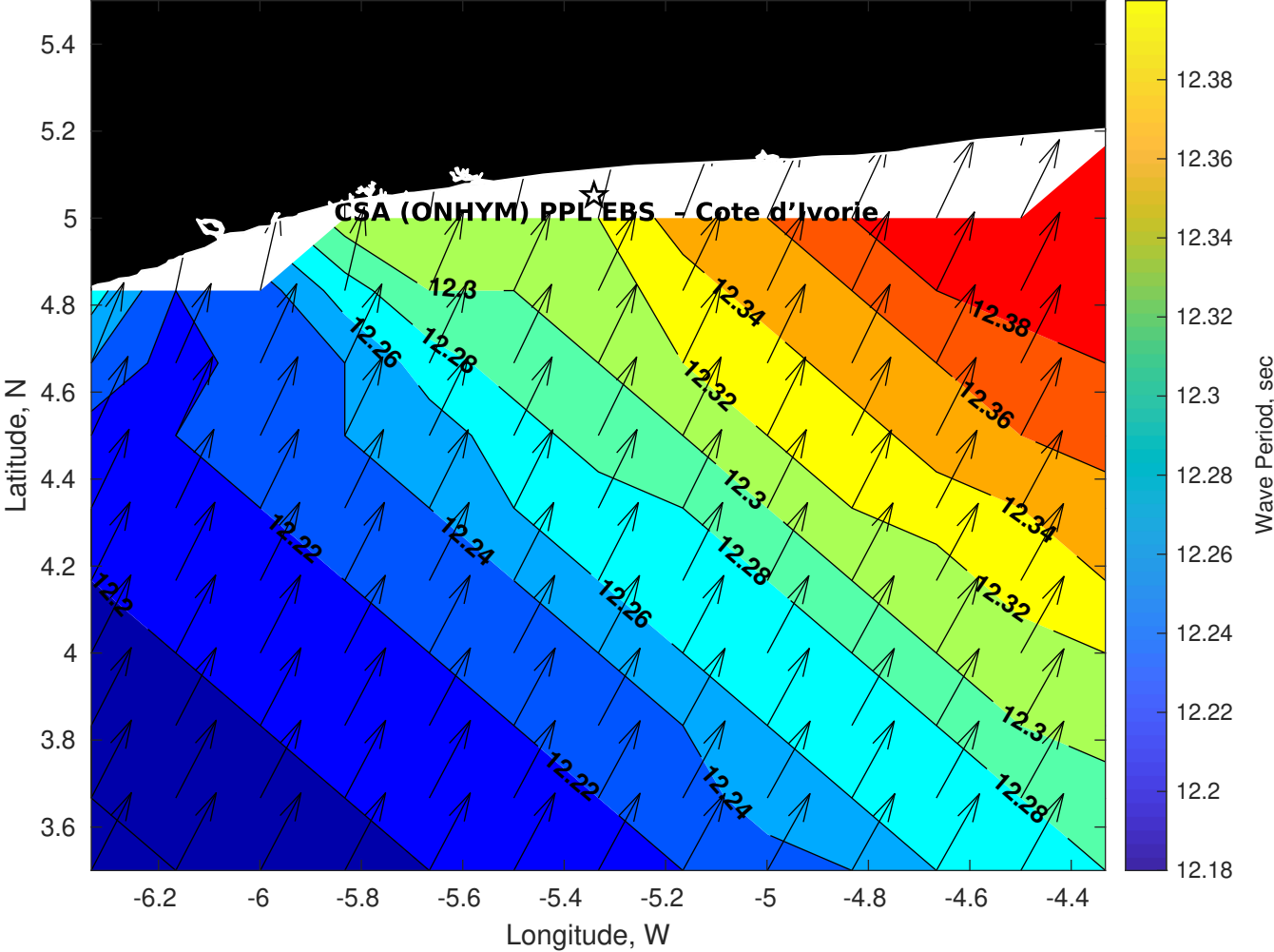
Wave Period (sec) for CSA (ONHYM) PPL EBS - Cote d'Ivoire at 23-Aug-2025 09:00:00
