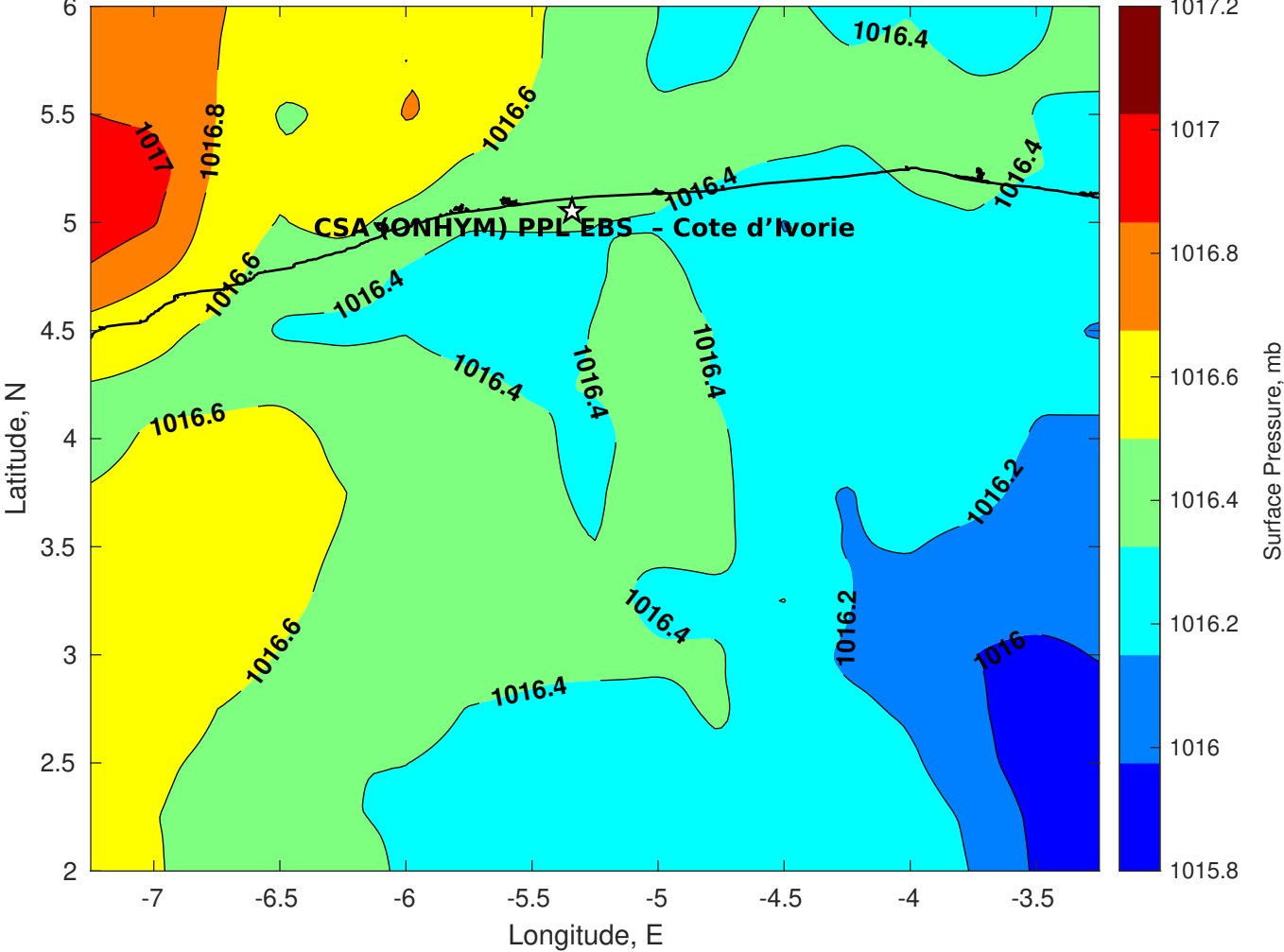
Surface Pressure (mb) for CSA (ONHYM) PPL EBS - Cote d'Ivoire at 25-Aug-2025 00:00:00
