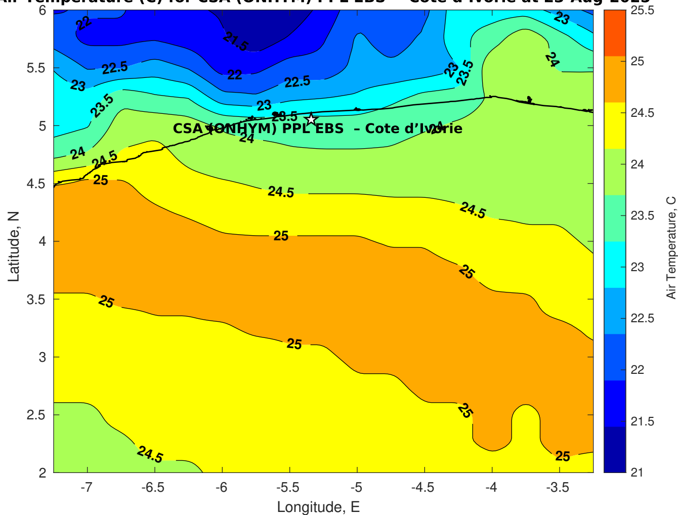
Air Temperature (C) for CSA (ONHYM) PPL EBS - Cote d'Ivoire at 23-Aug-2025
