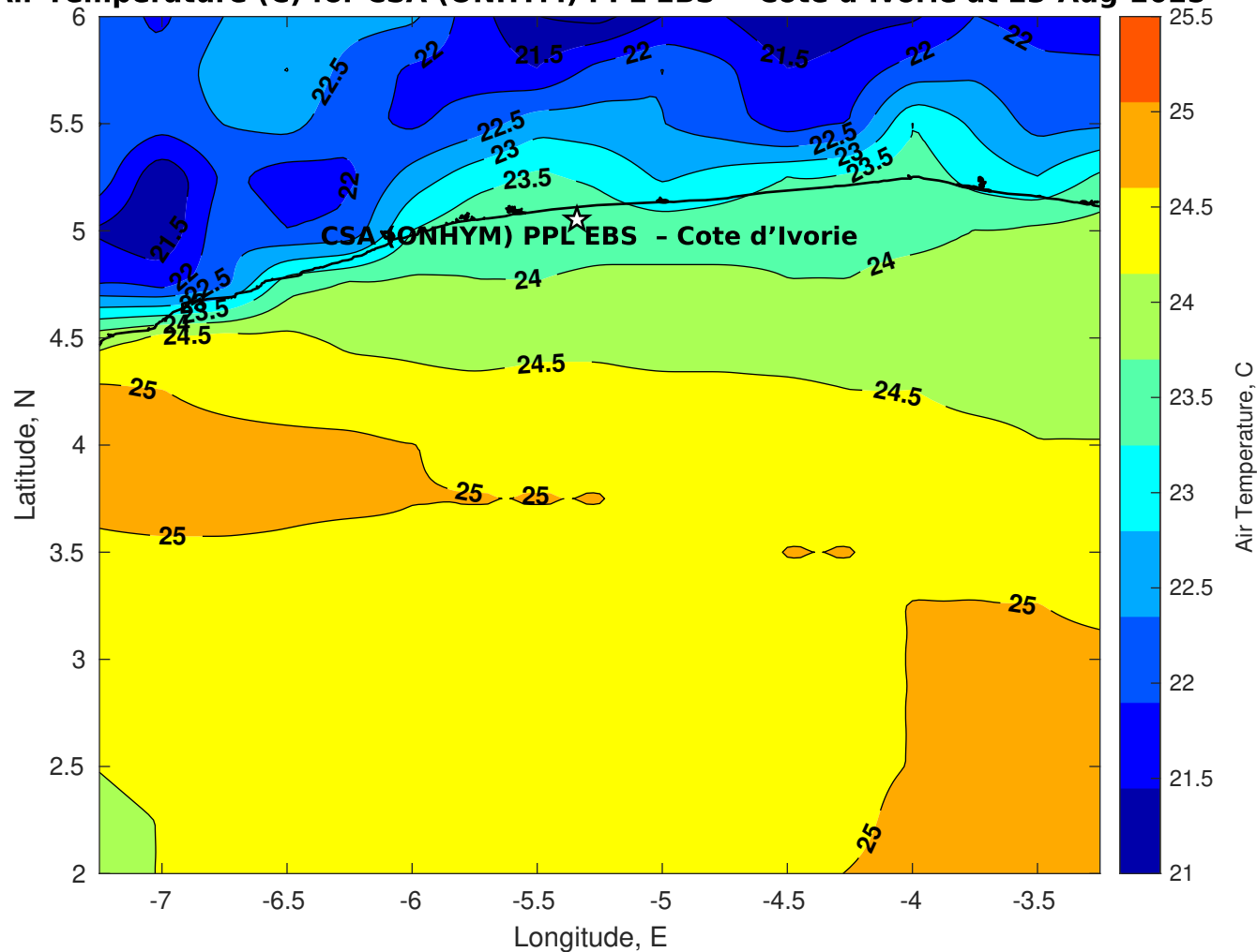
Air Temperature (C) for CSA (ONHYM) PPL EBS - Cote d'Ivoire at 23-Aug-2025
