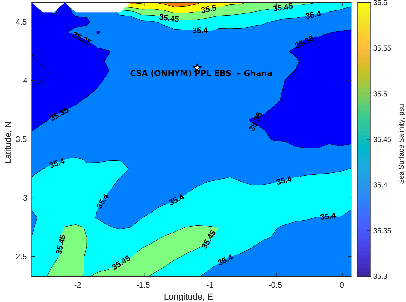
Surface Salinity for CSA (ONHYM) PPL EBS - Ghana at 22-Aug-2025 00:00:00
