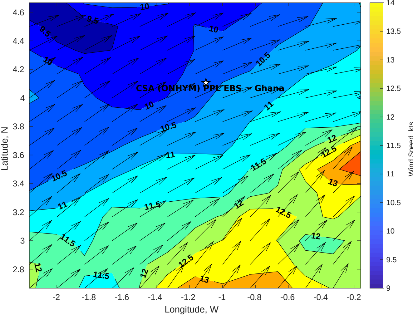
Winds (kts) for CSA (ONHYM) PPL EBS - Ghana at 23-Aug-2025 09:00:00
