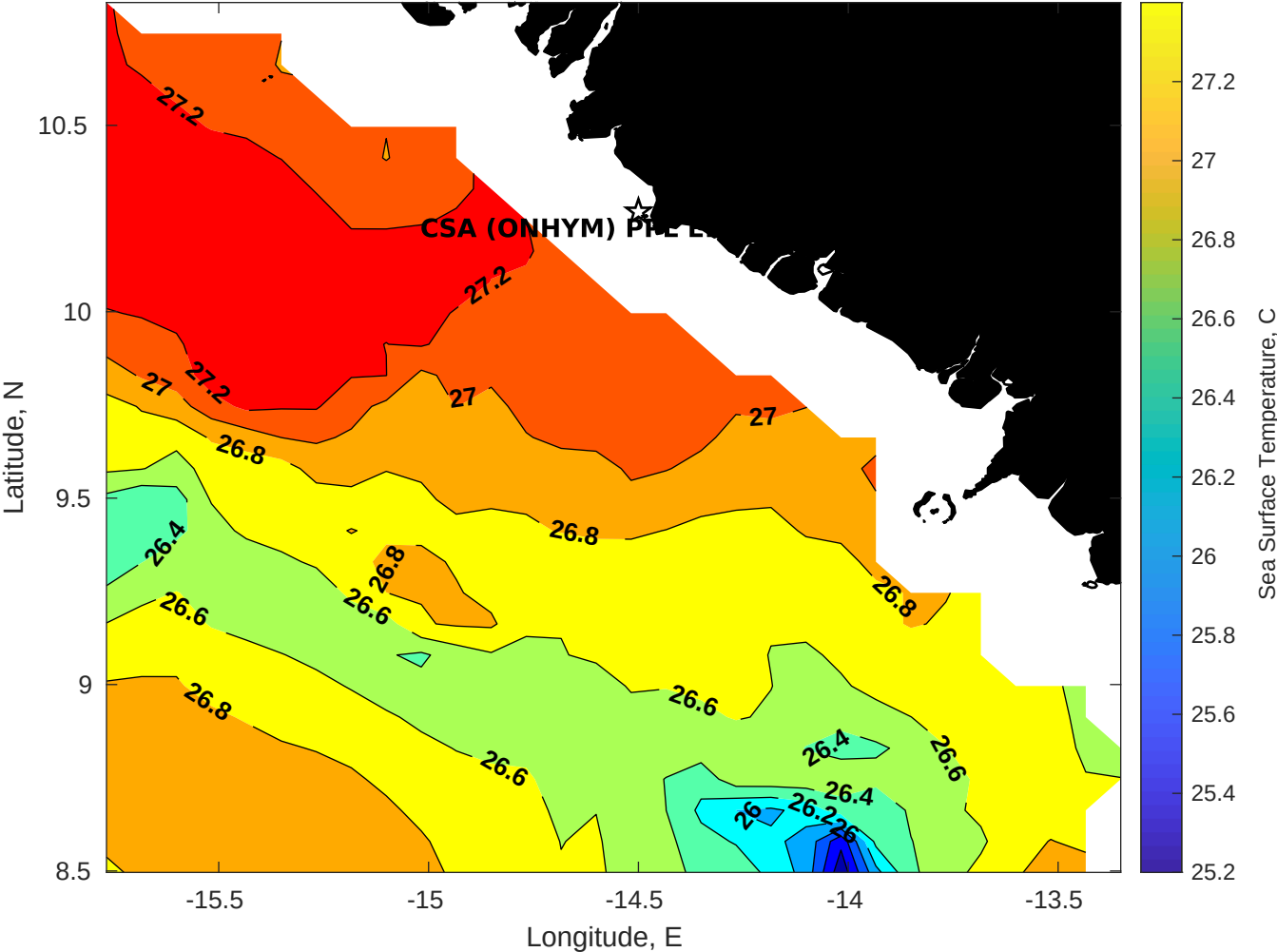
SST for CSA (ONHYM) PPL EBS - Guinea at 22-Aug-2025 00:00:00
