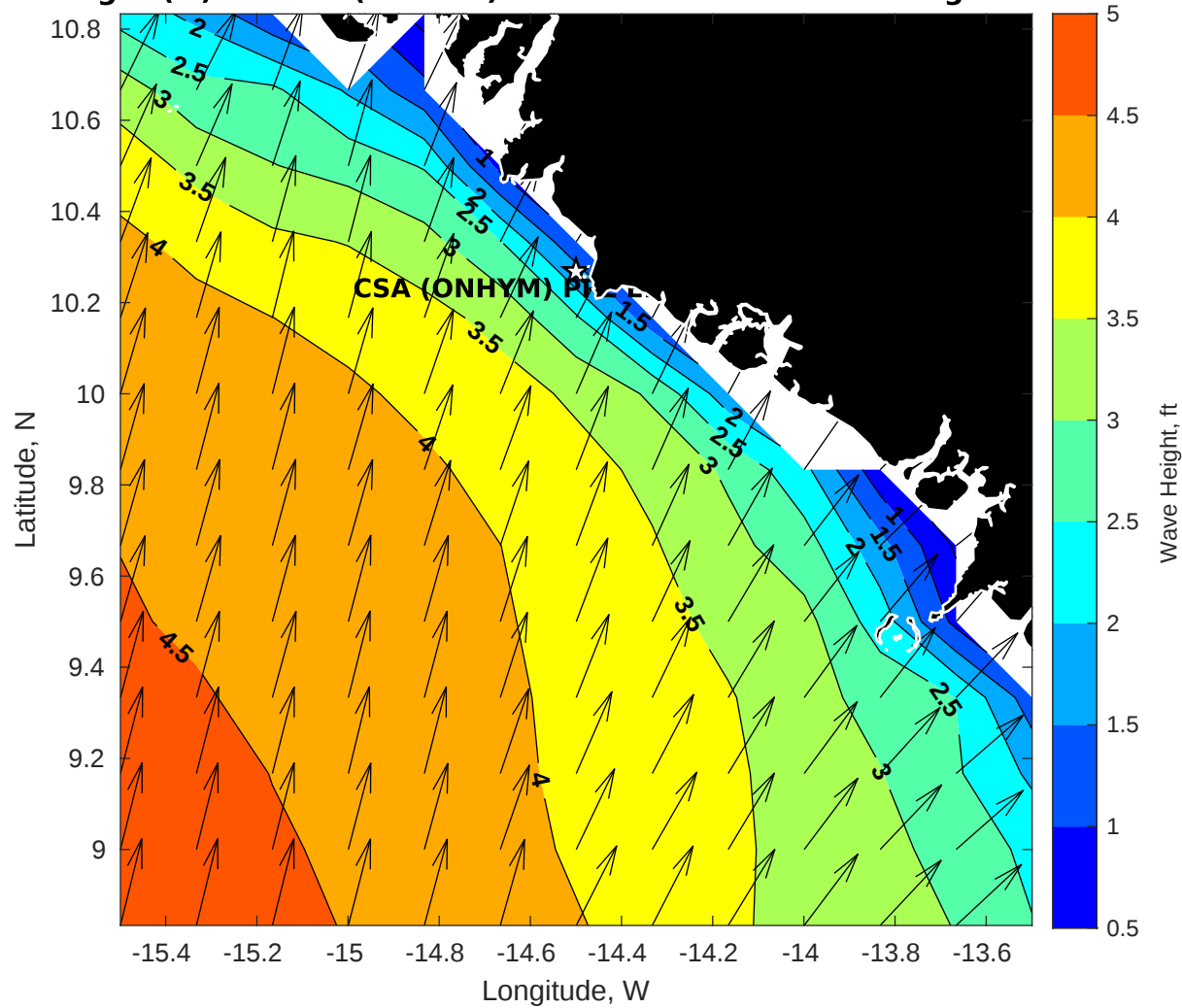
Wave Height (ft) for CSA (ONHYM) PPL EBS - Guinea at 23-Aug-2025 09:00:00
