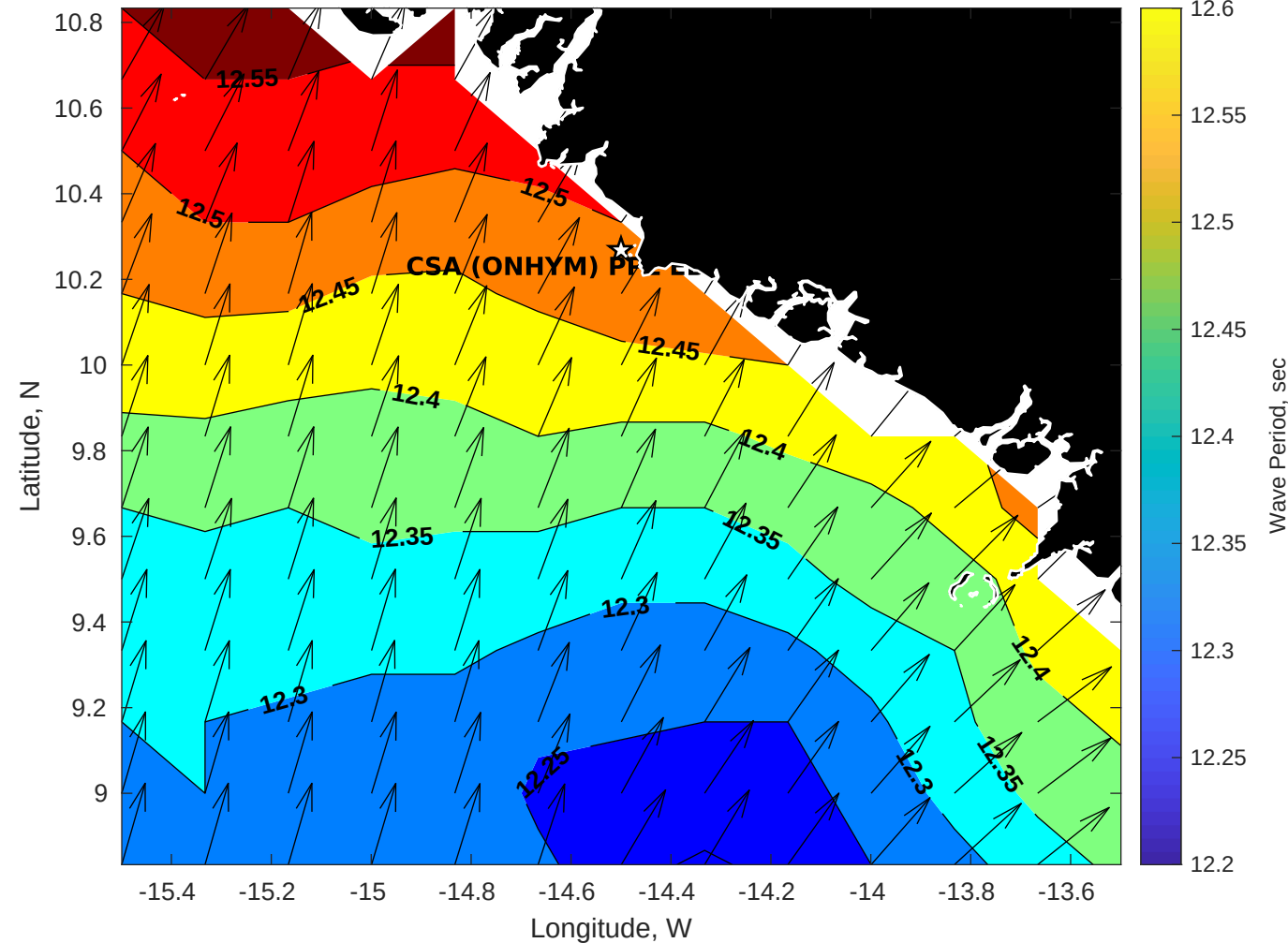
Wave Period (sec) for CSA (ONHYM) PPL EBS - Guinea at 23-Aug-2025 09:00:00
