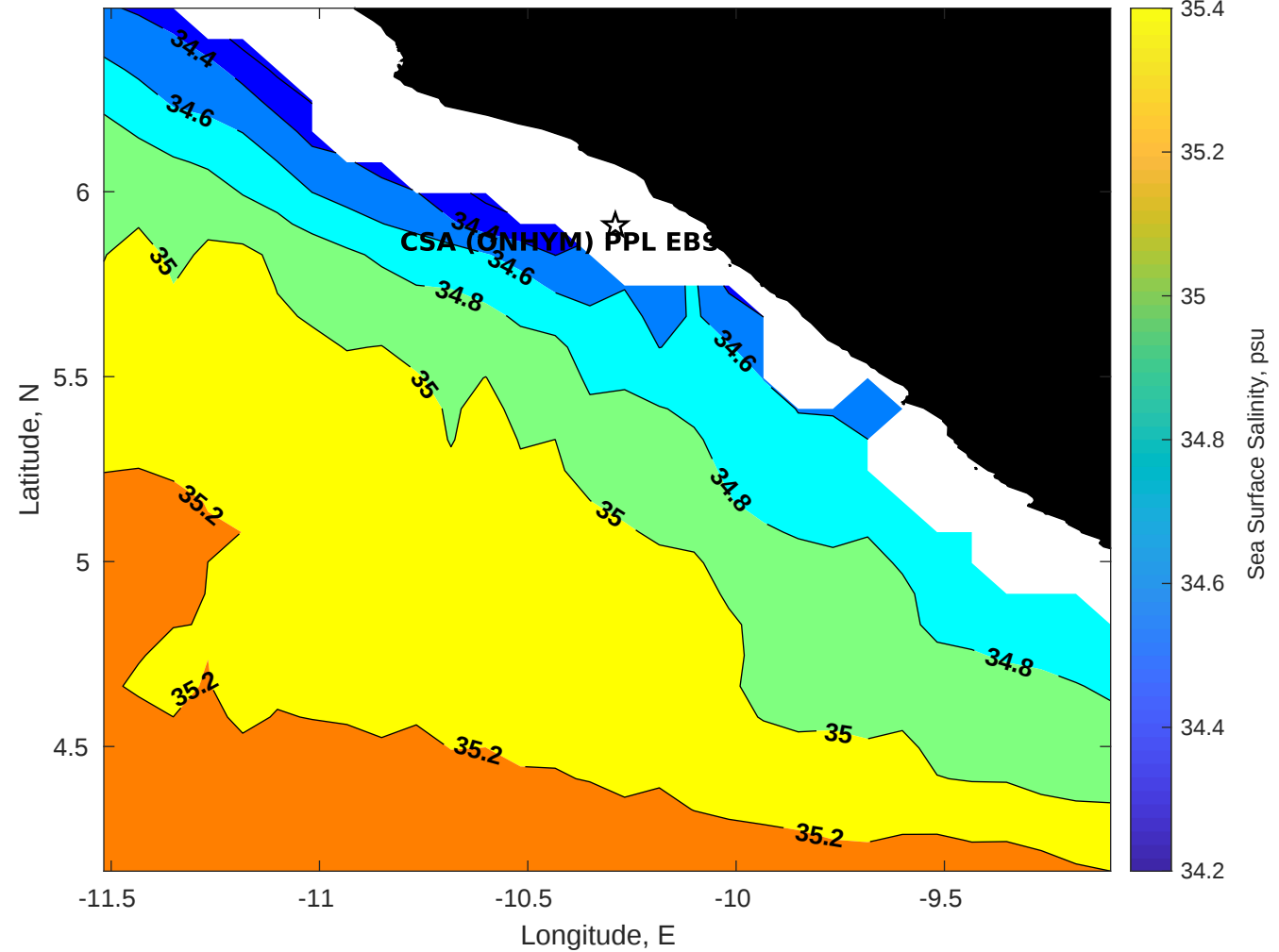
Surface Salinity for CSA (ONHYM) PPL EBS - Liberia at 22-Aug-2025 00:00:00
