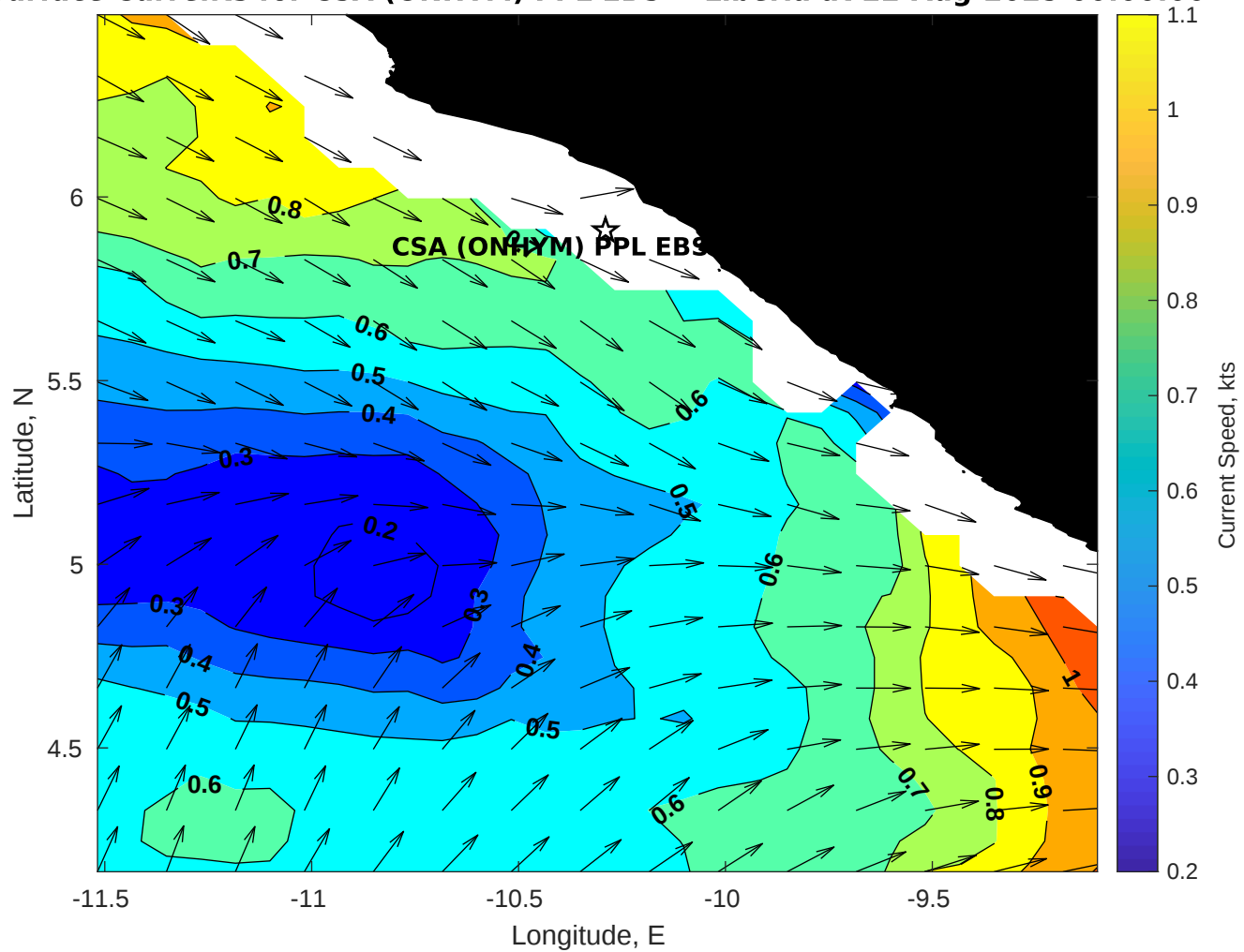
Surface Currents for CSA (ONHYM) PPL EBS - Liberia at 22-Aug-2025 00:00:00
