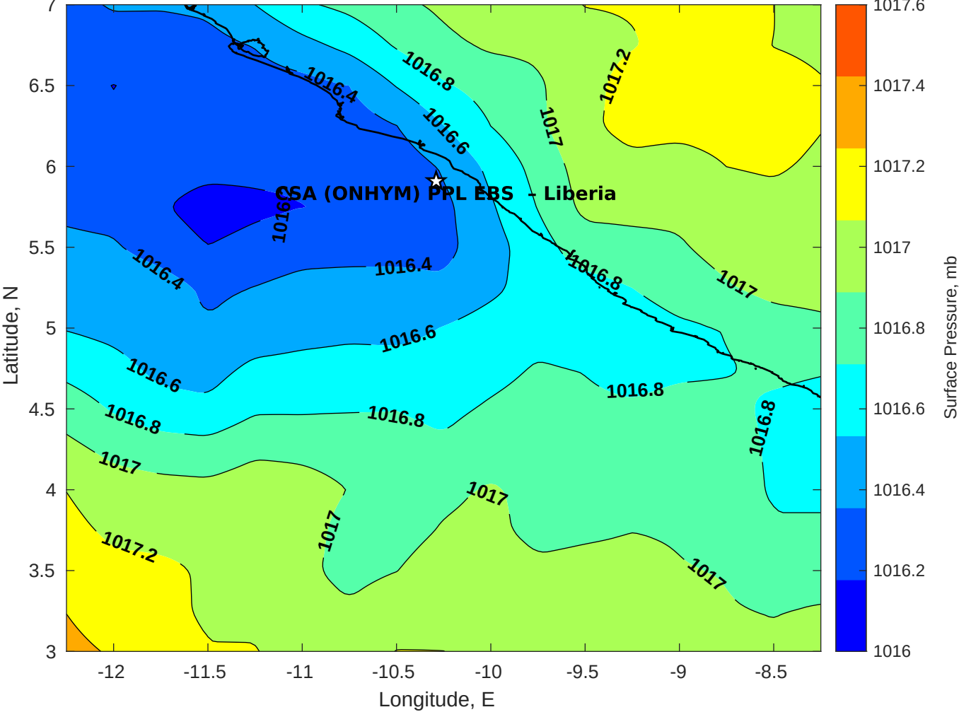
Surface Pressure (mb) for CSA (ONHYM) PPL EBS - Liberia at 25-Aug-2025 00:00:00
