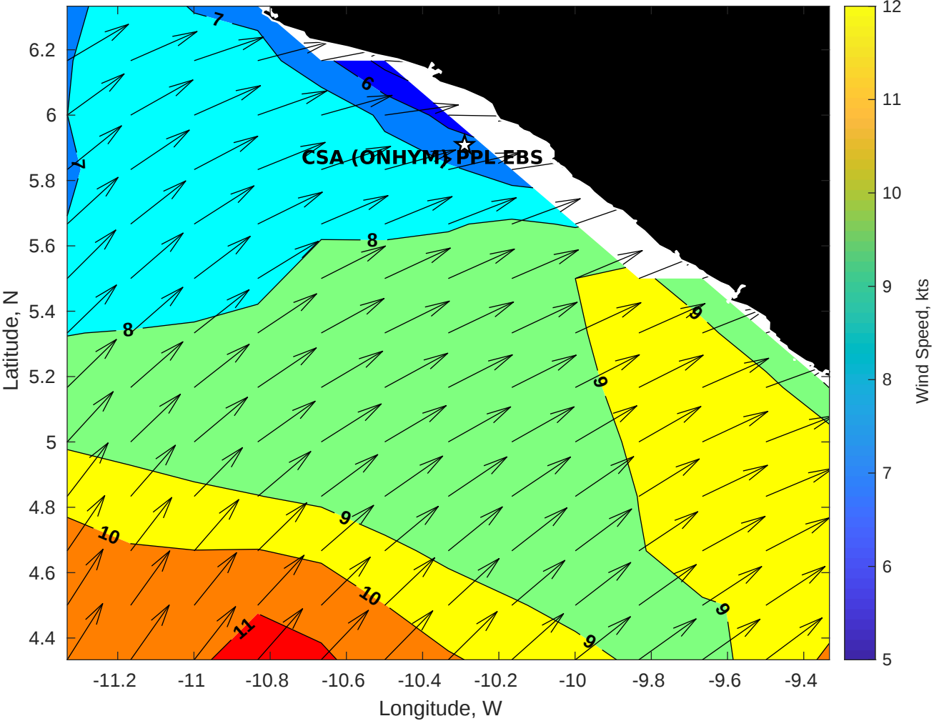
Winds (kts) for CSA (ONHYM) PPL EBS - Liberia at 23-Aug-2025 09:00:00
