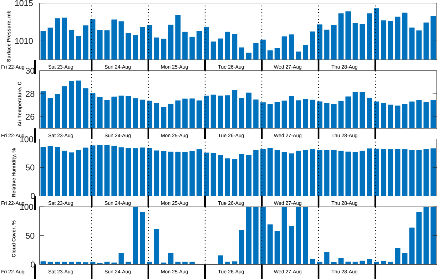
Met Forecast for CSA (ONHYM) PPL EBS - Mauritania from 23-Aug-2025 00:00:00 to 30-Aug-2025 00:00:00
