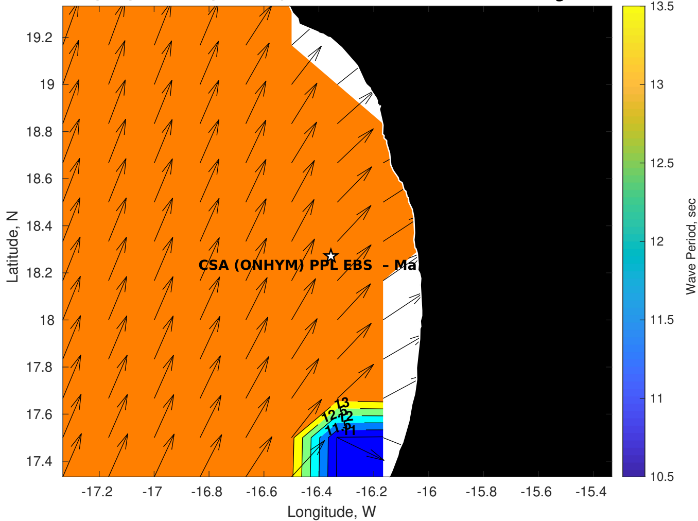
Wave Period (sec) for CSA (ONHYM) PPL EBS - Mauritania at 23-Aug-2025 09:00:00
