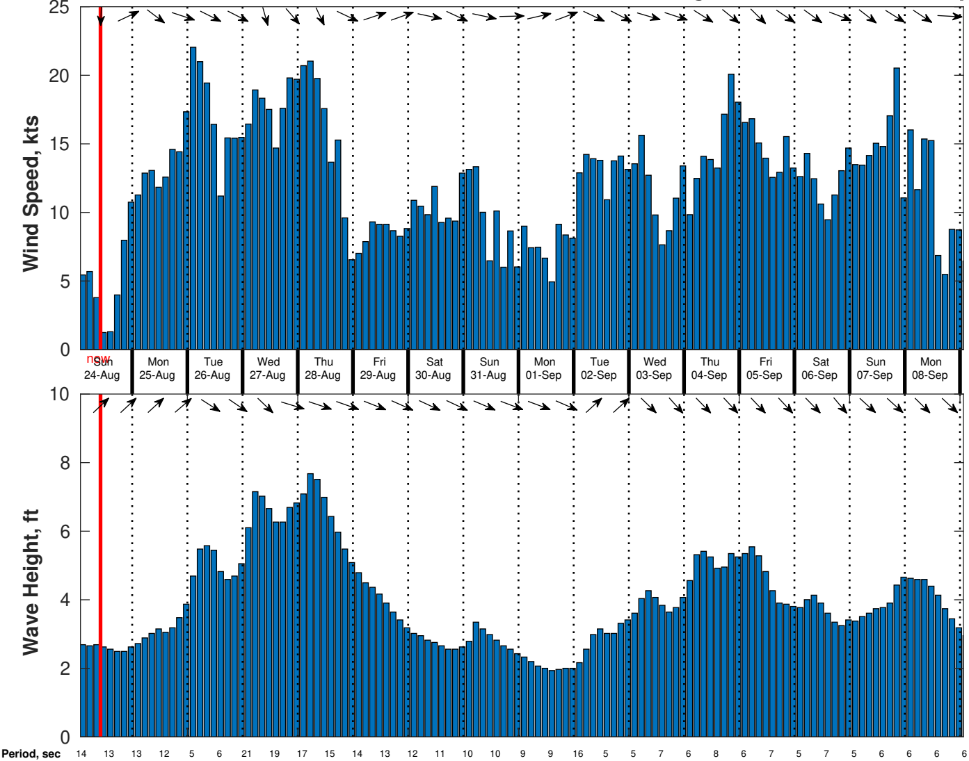
Wind & Wave Forecast for CSA (ONHYM) PPL EBS - Mauritania from 23-Aug-2025 01:00:00 to 08-Sep-2025 01:00:00
