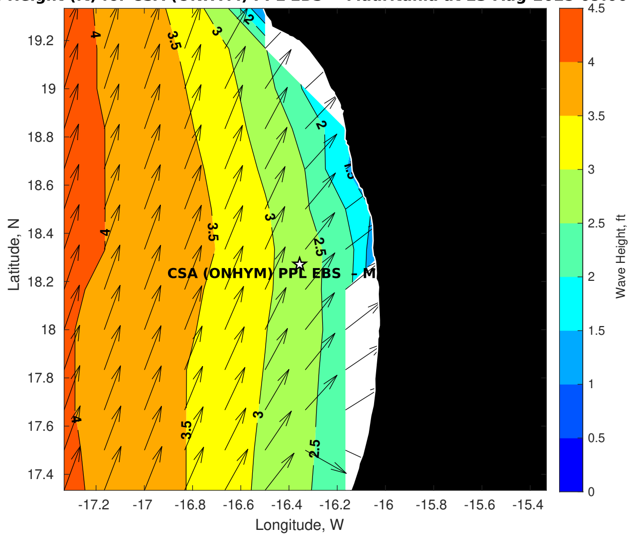
Wave Height (ft) for CSA (ONHYM) PPL EBS - Mauritania at 23-Aug-2025 09:00:00
