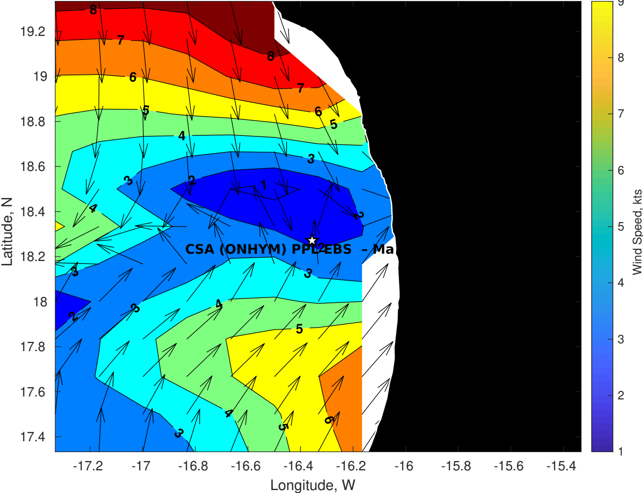
Winds (kts) for CSA (ONHYM) PPL EBS - Mauritania at 23-Aug-2025 09:00:00
