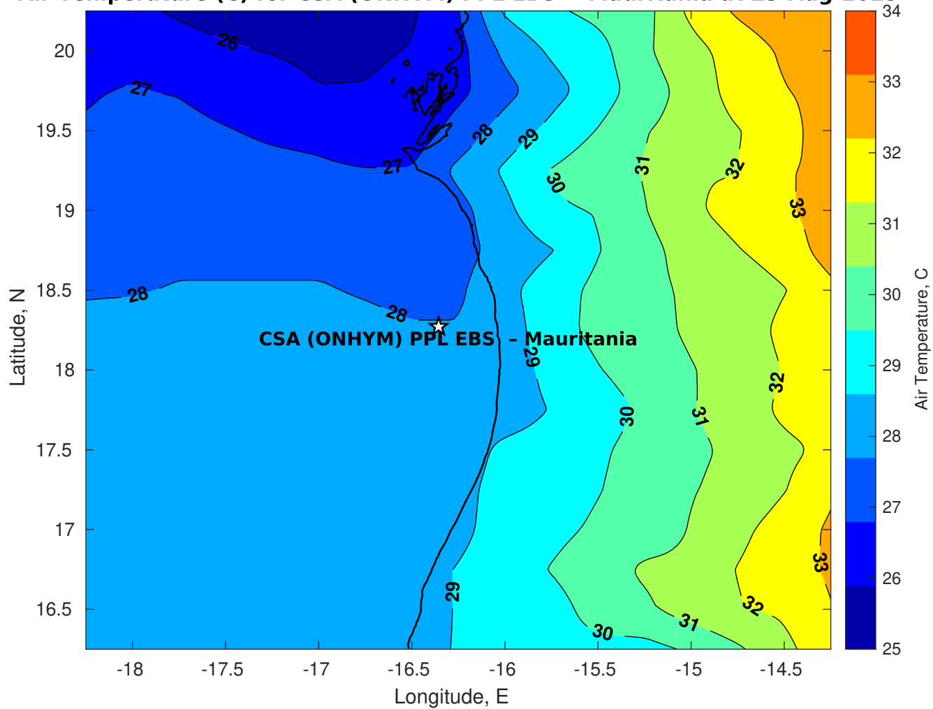
Air Temperature (C) for CSA (ONHYM) PPL EBS - Mauritania at 23-Aug-2025
