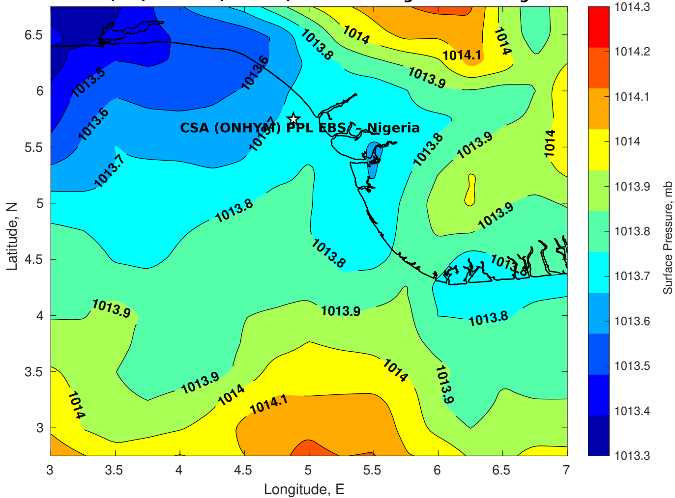
Surface Pressure (mb) for CSA (ONHYM) PPL EBS - Nigeria at 23-Aug-2025 00:00:00
