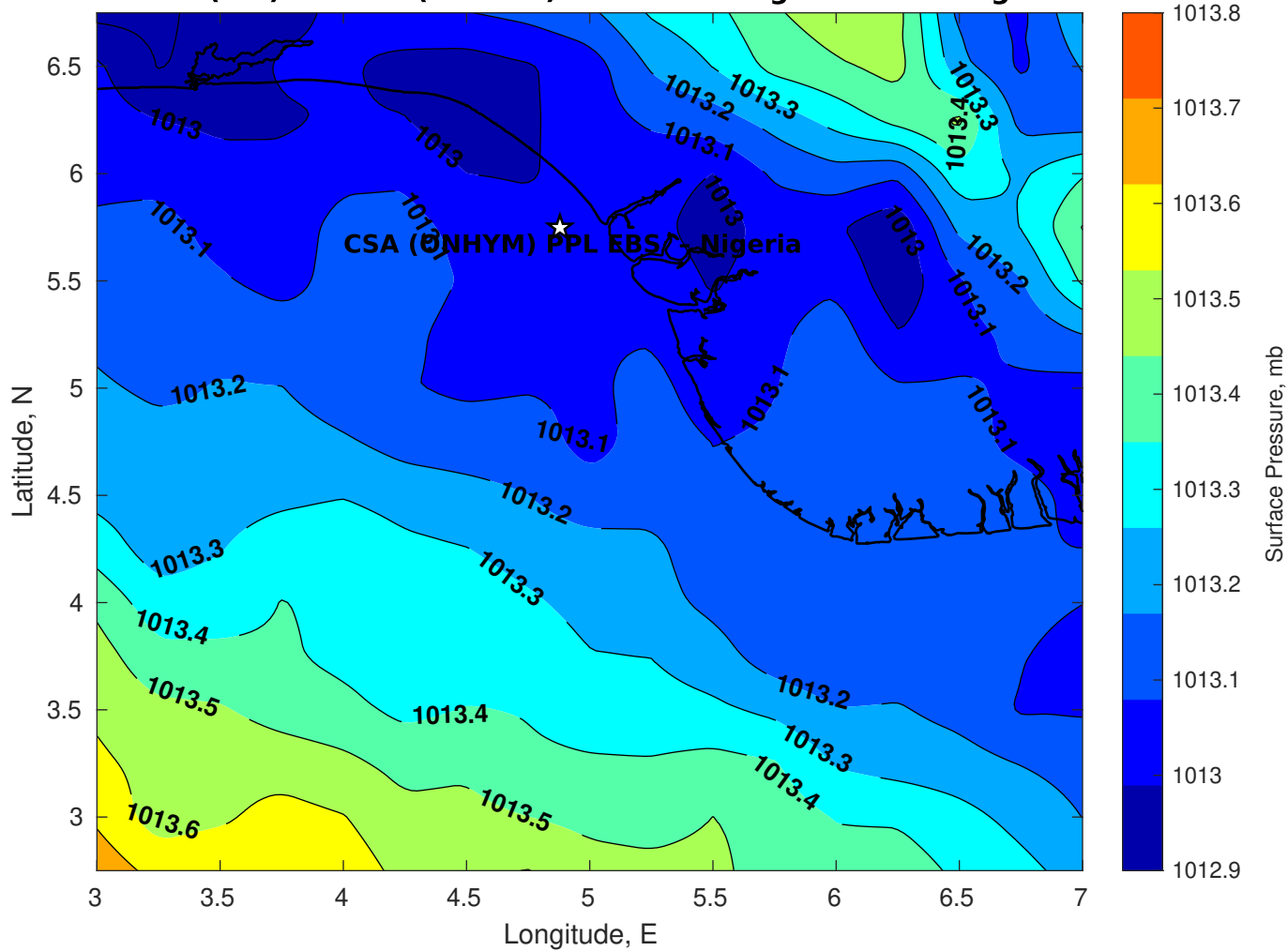
Surface Pressure (mb) for CSA (ONHYM) PPL EBS - Nigeria at 24-Aug-2025 00:00:00
