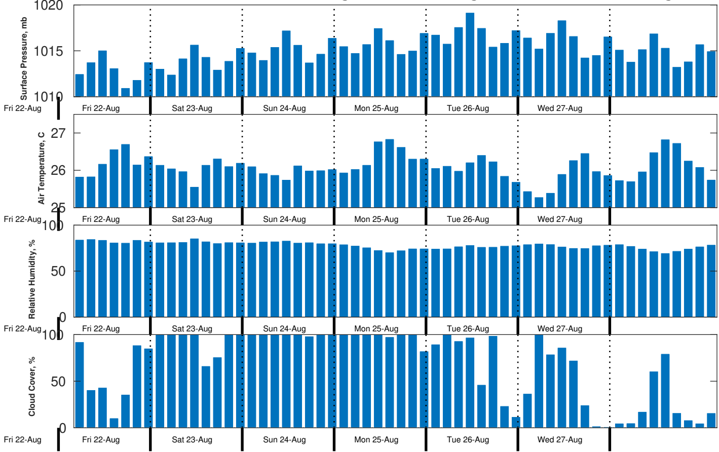
Met Forecast for CSA (ONHYM) PPL EBS - Nigeria from 23-Aug-2025 00:00:00 to 30-Aug-2025 00:00:00
