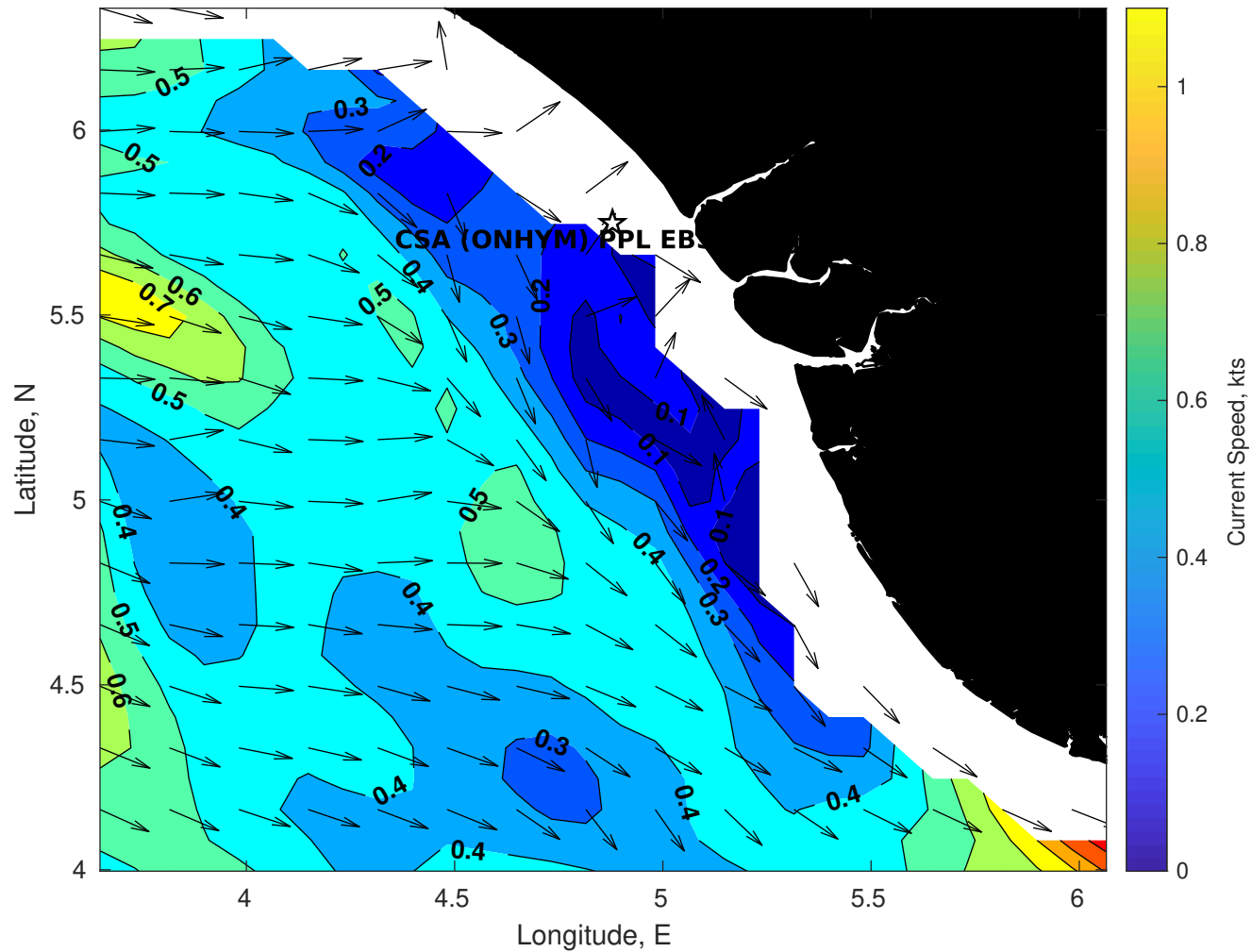
Surface Currents for CSA (ONHYM) PPL EBS - Nigeria at 22-Aug-2025 00:00:00
