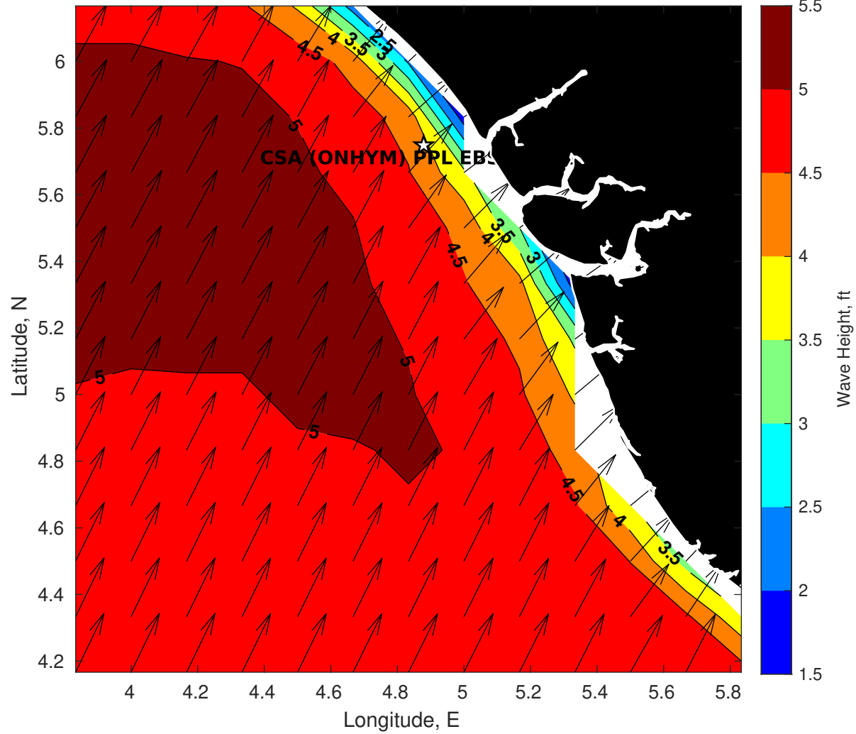
Wave Height (ft) for CSA (ONHYM) PPL EBS - Nigeria at 23-Aug-2025 09:00:00
