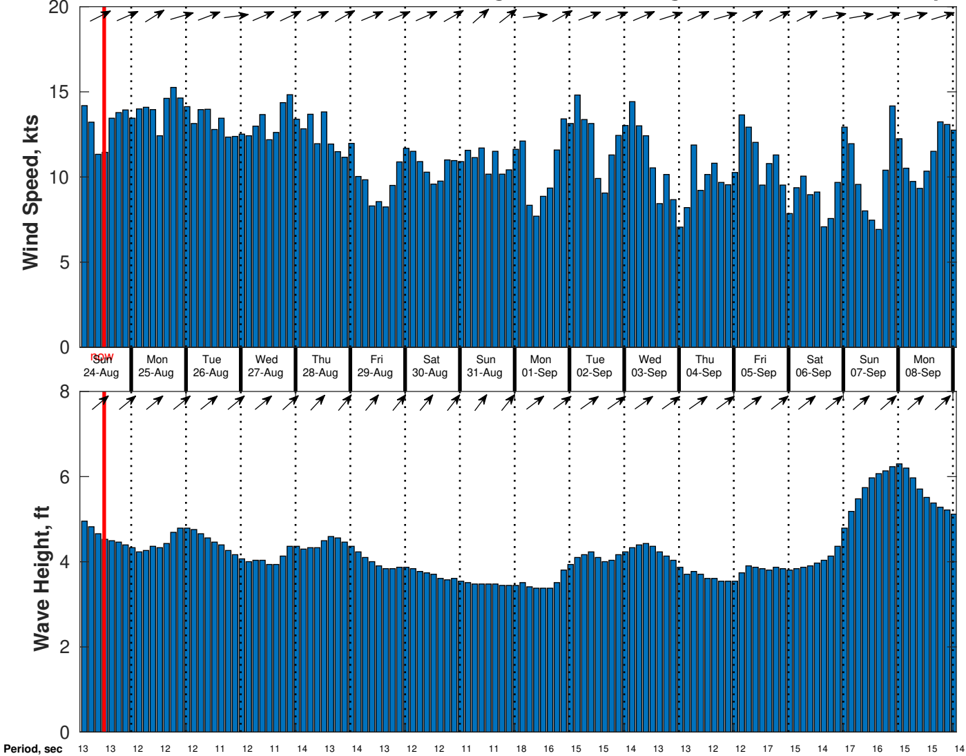
Wind & Wave Forecast for CSA (ONHYM) PPL EBS - Nigeria from 23-Aug-2025 02:00:00 to 08-Sep-2025 02:00:00
