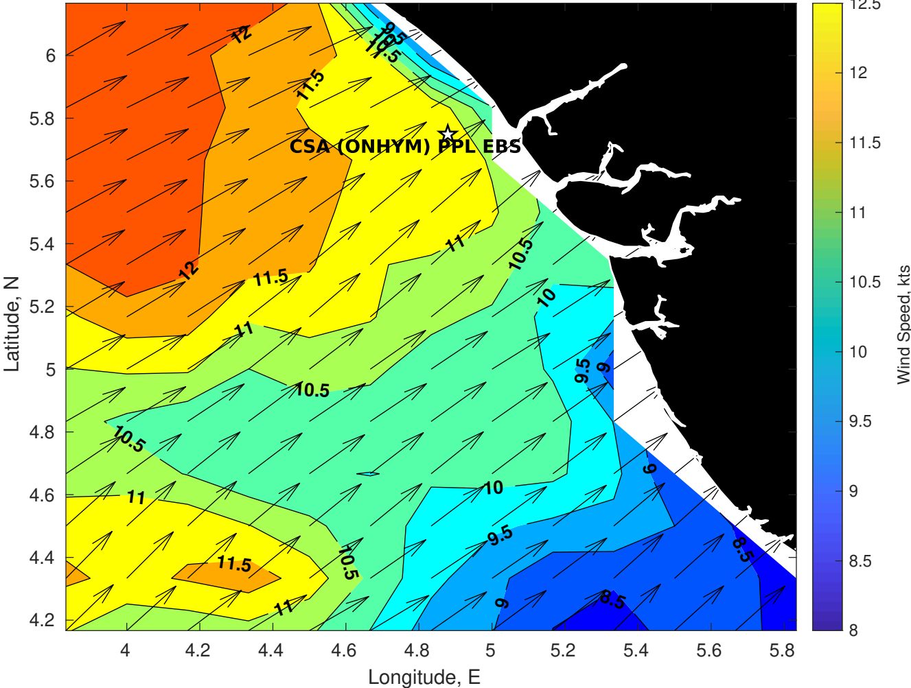
Winds (kts) for CSA (ONHYM) PPL EBS - Nigeria at 23-Aug-2025 09:00:00
