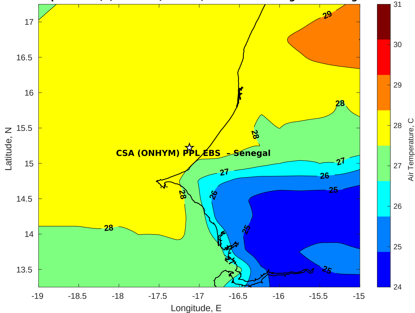
Air Temperature (C) for CSA (ONHYM) PPL EBS - Senegal at 23-Aug-2025
