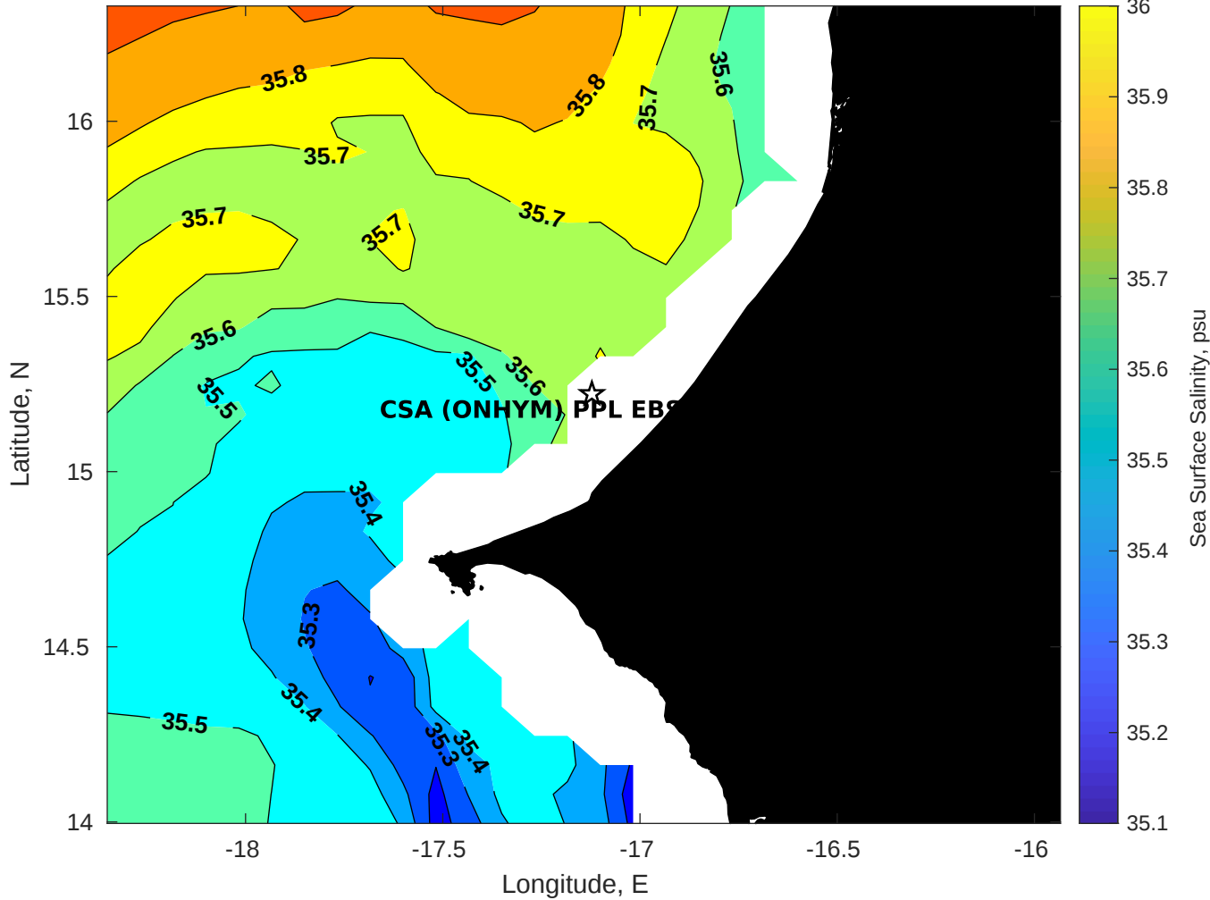
Surface Salinity for CSA (ONHYM) PPL EBS - Senegal at 22-Aug-2025 00:00:00
