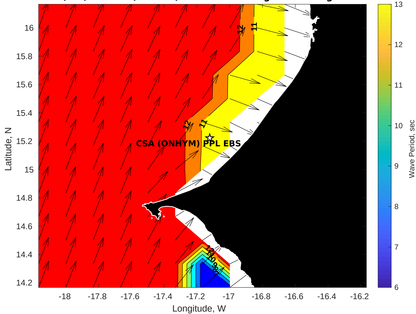
Wave Period (sec) for CSA (ONHYM) PPL EBS - Senegal at 23-Aug-2025 09:00:00
