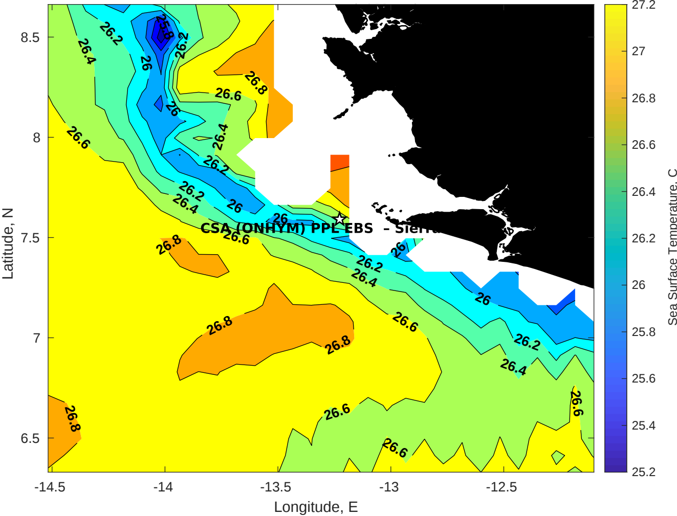
SST for CSA (ONHYM) PPL EBS - Sierra Leone at 22-Aug-2025 00:00:00
