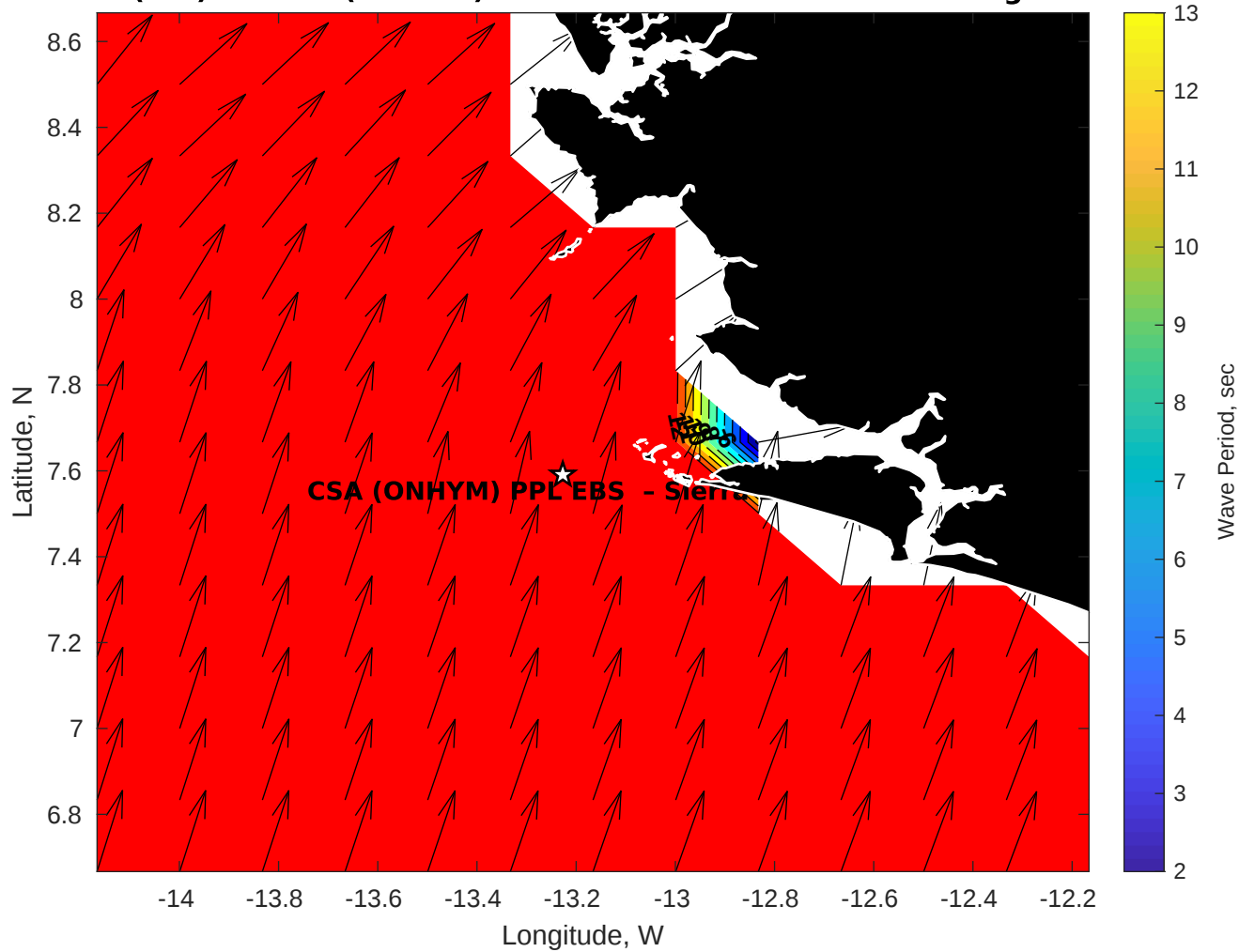
Wave Period (sec) for CSA (ONHYM) PPL EBS - Sierra Leone at 23-Aug-2025 09:00:00
