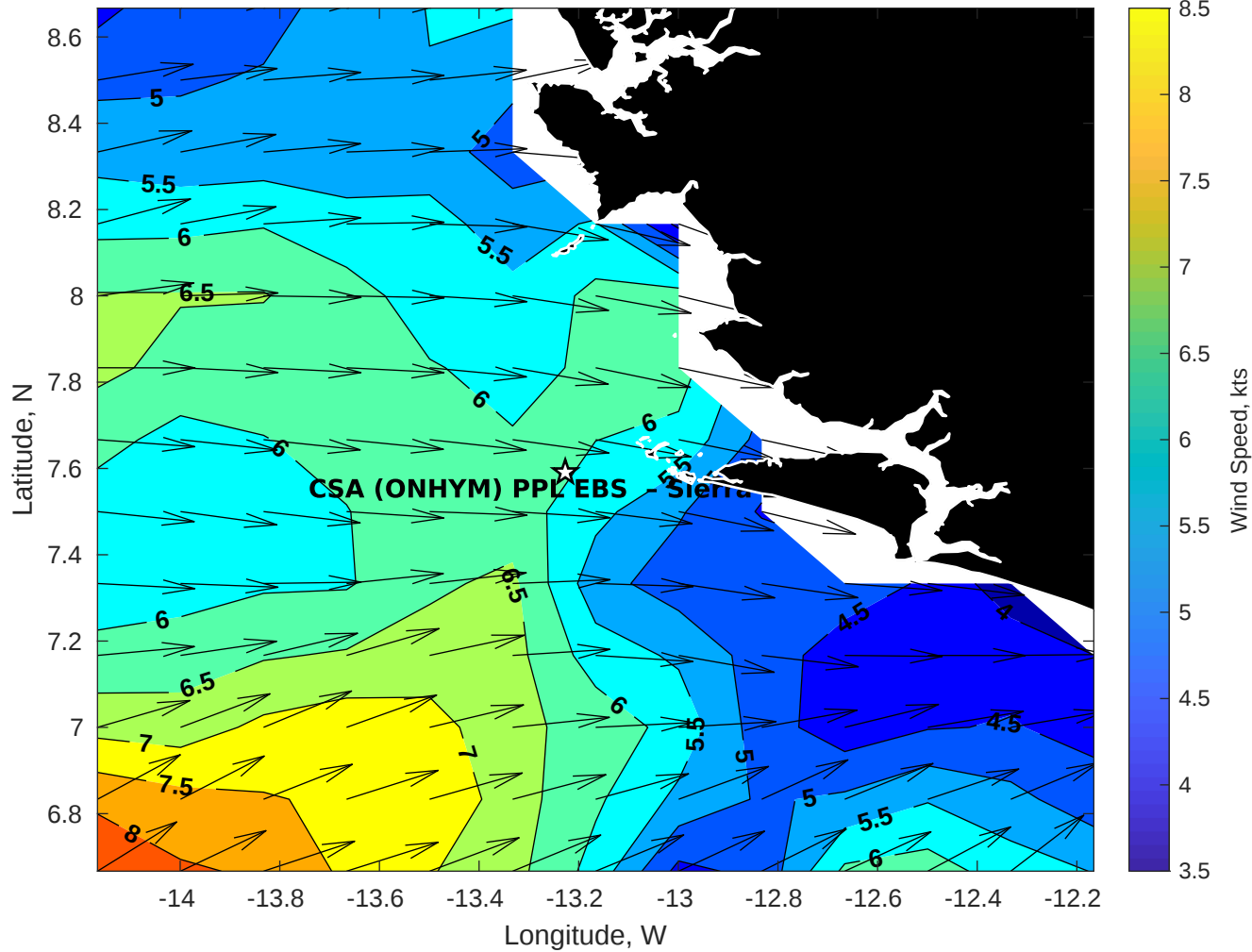
Winds (kts) for CSA (ONHYM) PPL EBS - Sierra Leone at 23-Aug-2025 09:00:00
