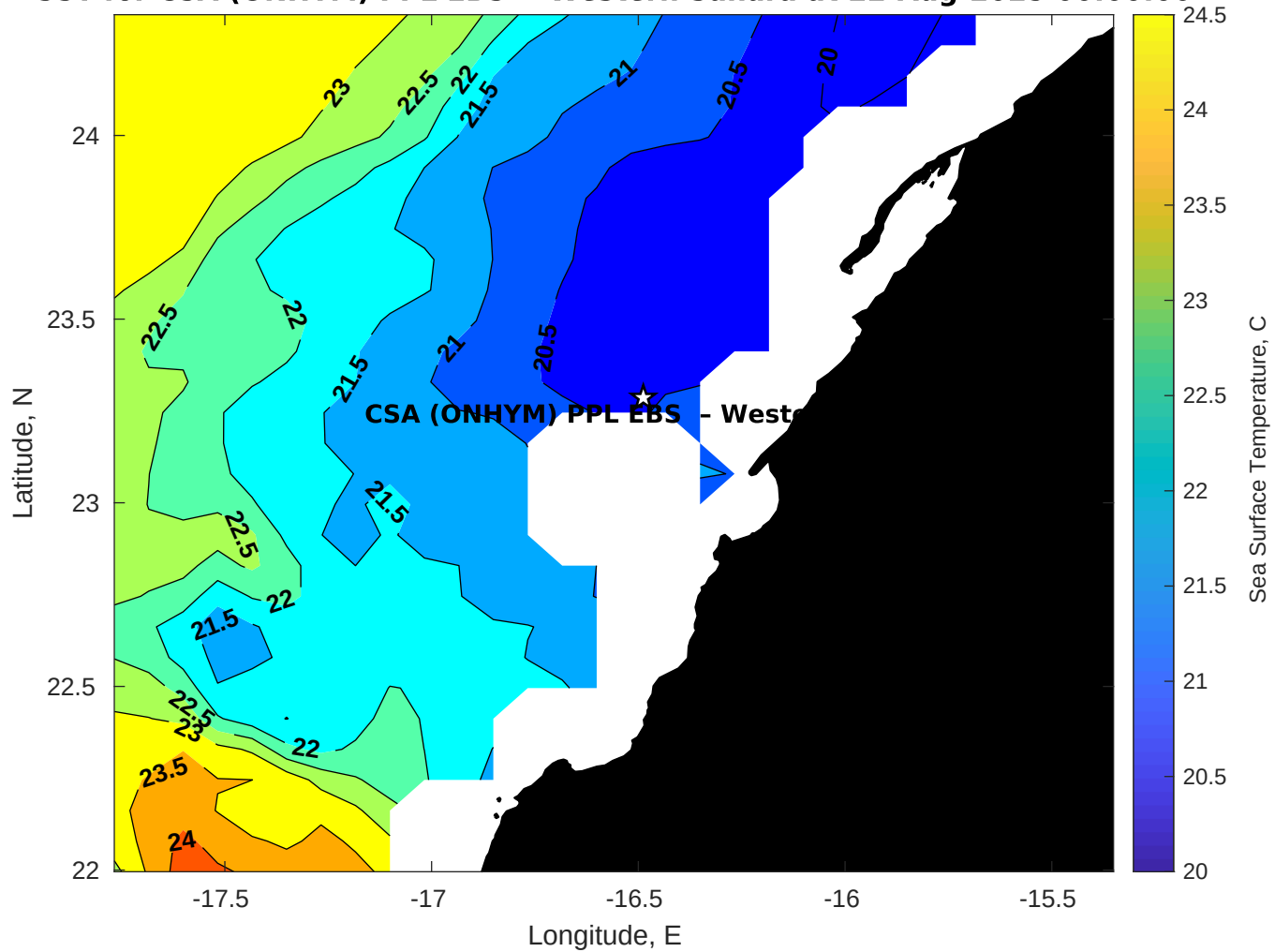
SST for CSA (ONHYM) PPL EBS - Western Sahara at 22-Aug-2025 00:00:00
