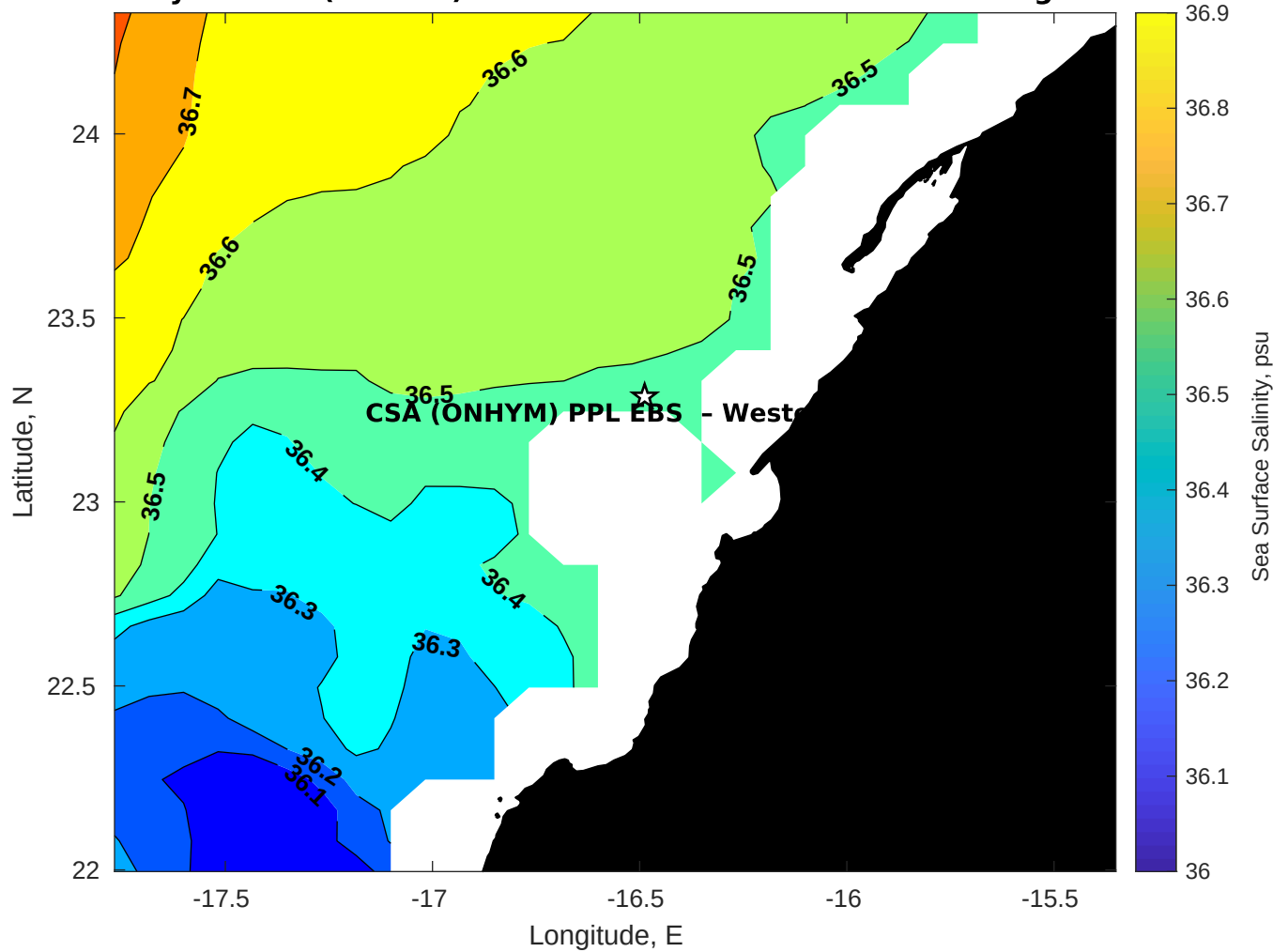
Surface Salinity for CSA (ONHYM) PPL EBS - Western Sahara at 22-Aug-2025 00:00:00
