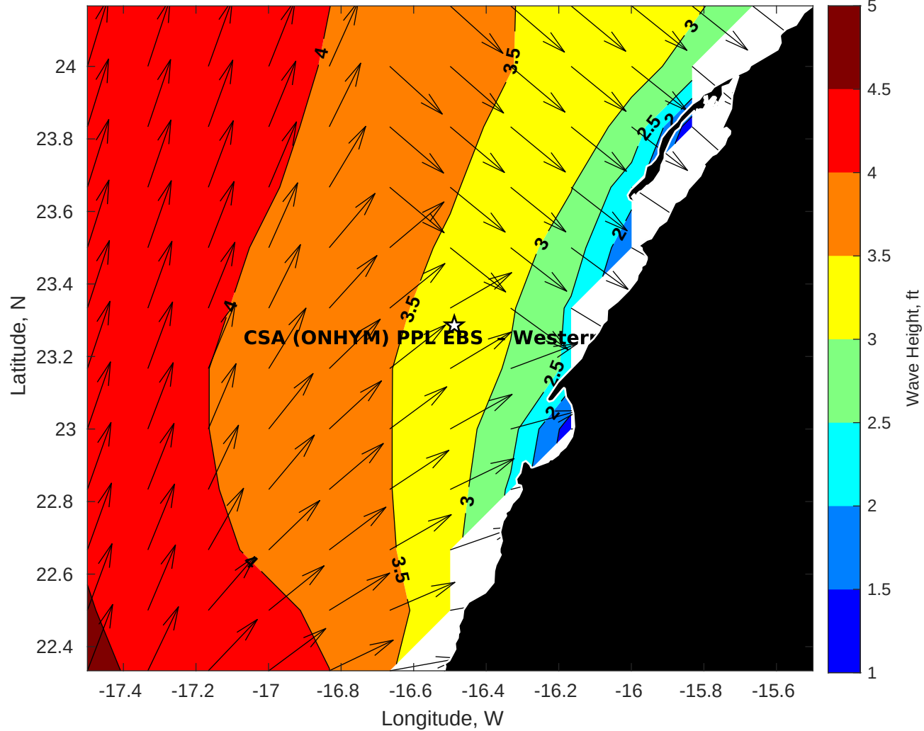
Wave Height (ft) for CSA (ONHYM) PPL EBS - Western Sahara at 23-Aug-2025 09:00:00
