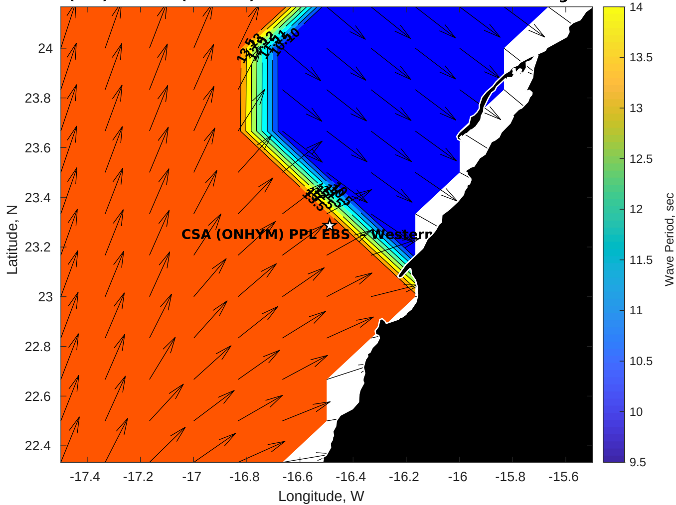
Wave Period (sec) for CSA (ONHYM) PPL EBS - Western Sahara at 23-Aug-2025 09:00:00
