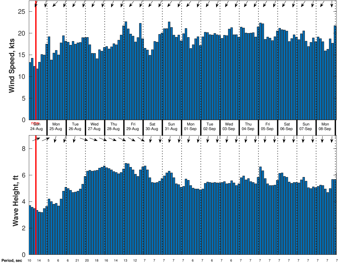
Wind & Wave Forecast for CSA (ONHYM) PPL EBS - Western Sahara from 23-Aug-2025 01:00:00 to 08-Sep-2025 01:00:00
