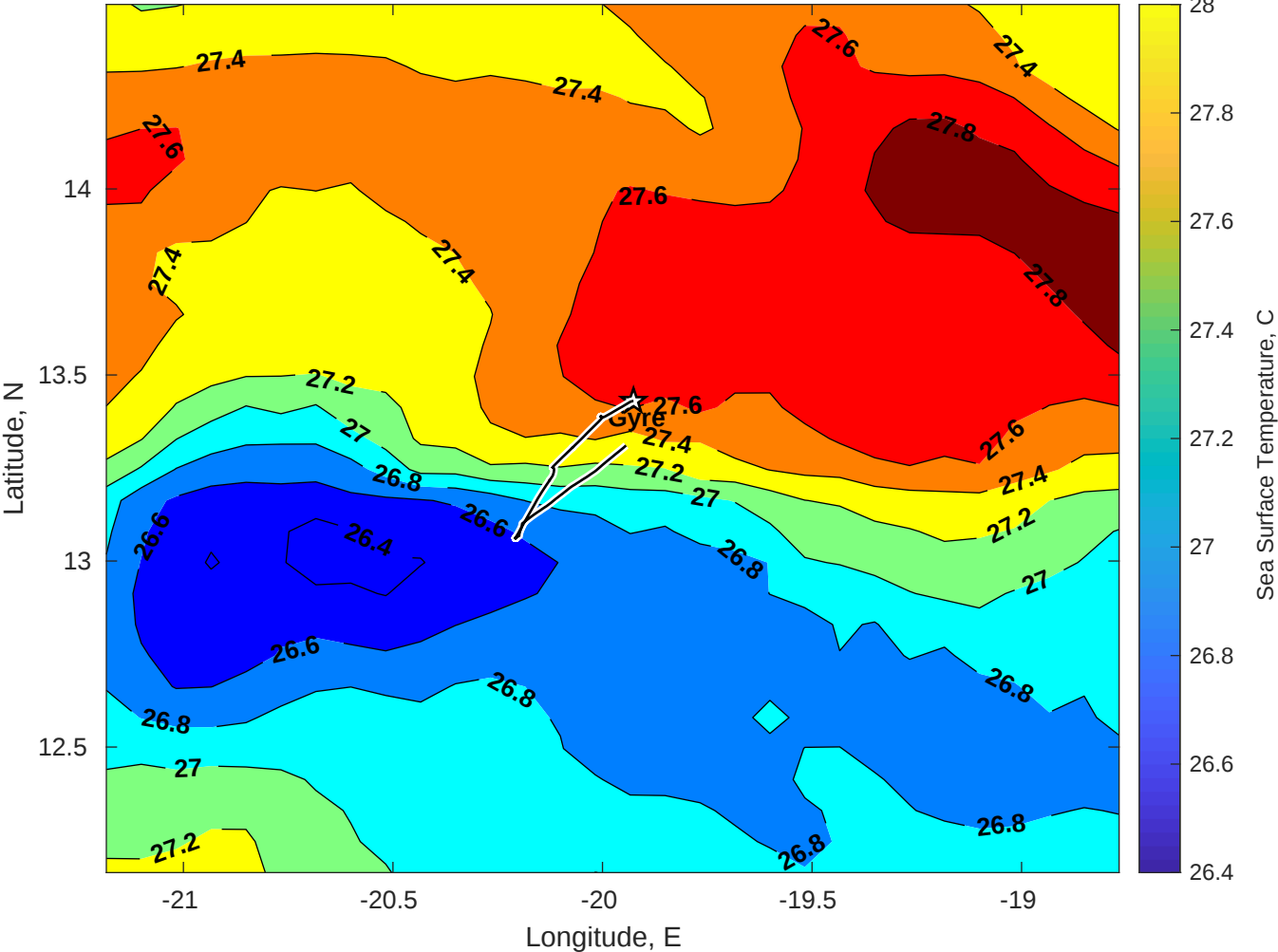
SST for Gyre at 22-Aug-2025 00:00:00
