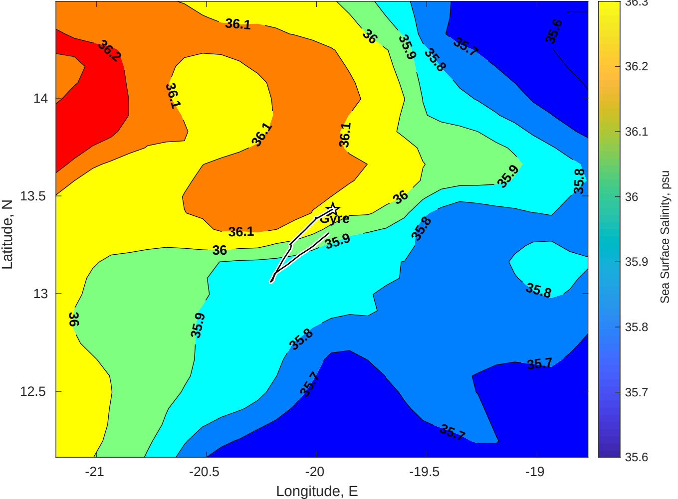
Surface Salinity for Gyre at 22-Aug-2025 00:00:00
