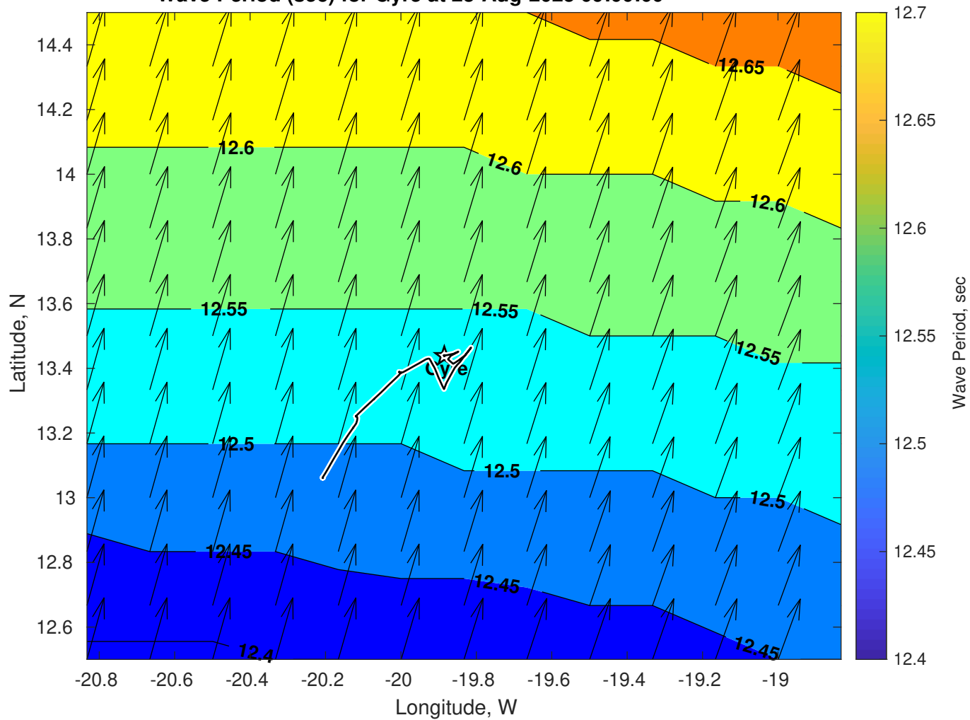
Wave Period (sec) for Gyre at 23-Aug-2025 09:00:00
