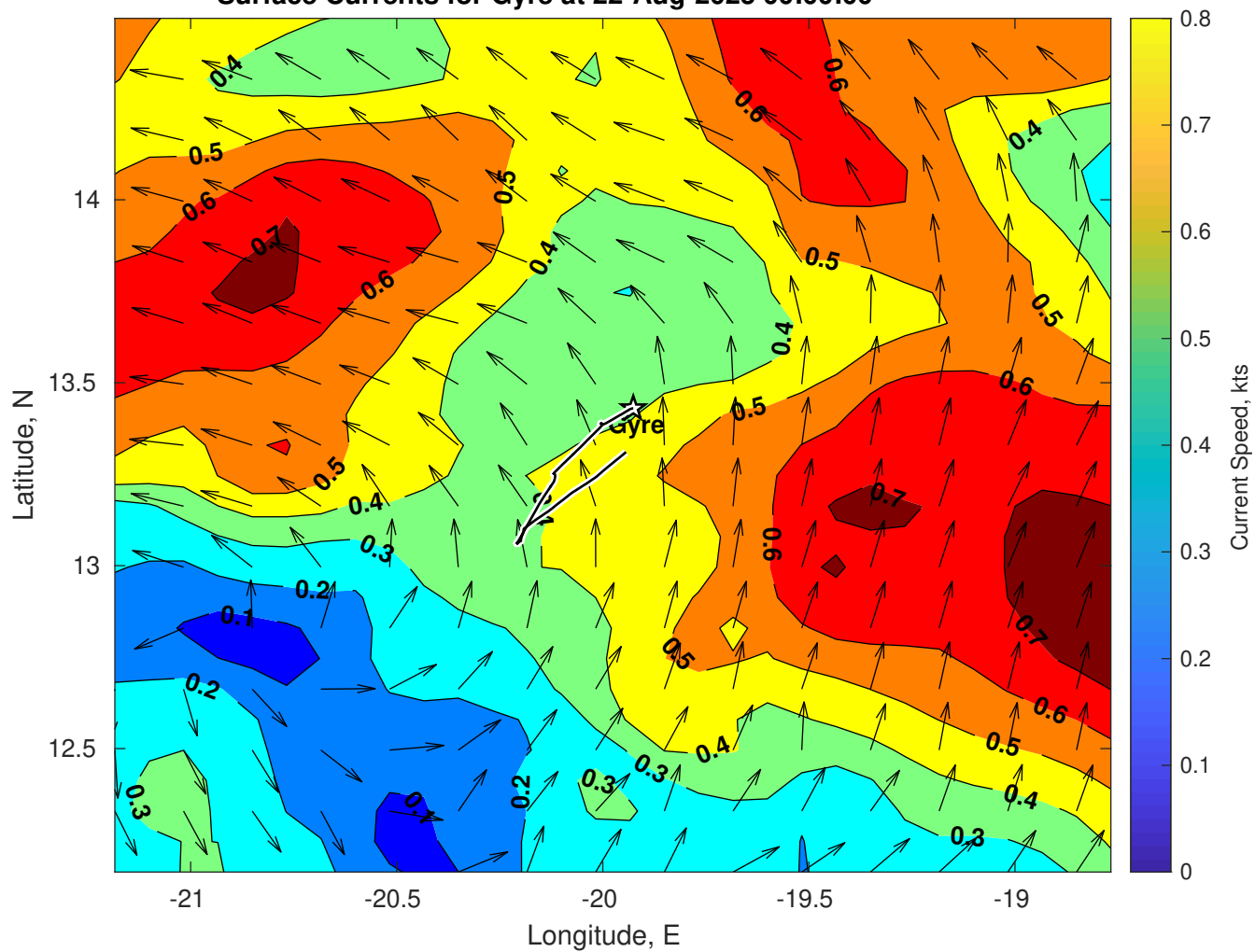
Surface Currents for Gyre at 22-Aug-2025 00:00:00
