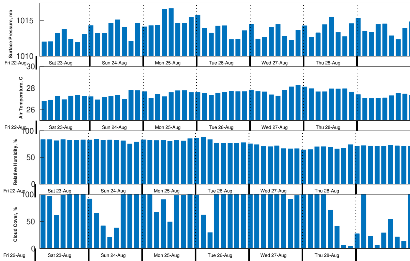
Met Forecast for Gyre from 22-Aug-2025 23:00:00 to 29-Aug-2025 23:00:00
