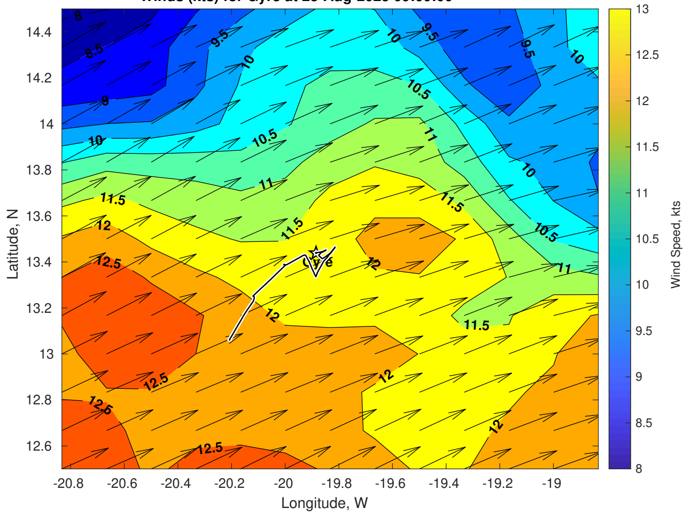
Winds (kts) for Gyre at 23-Aug-2025 09:00:00
