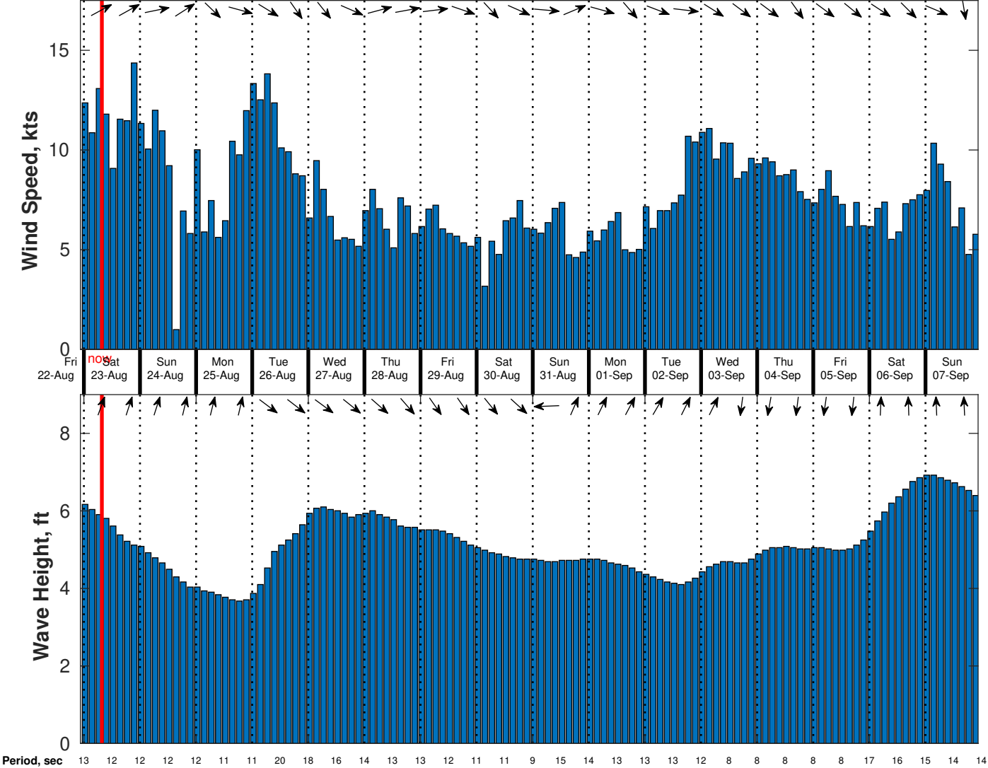
Wind & Wave Forecast for Gyre from 22-Aug-2025 23:00:00 to 07-Sep-2025 23:00:00
