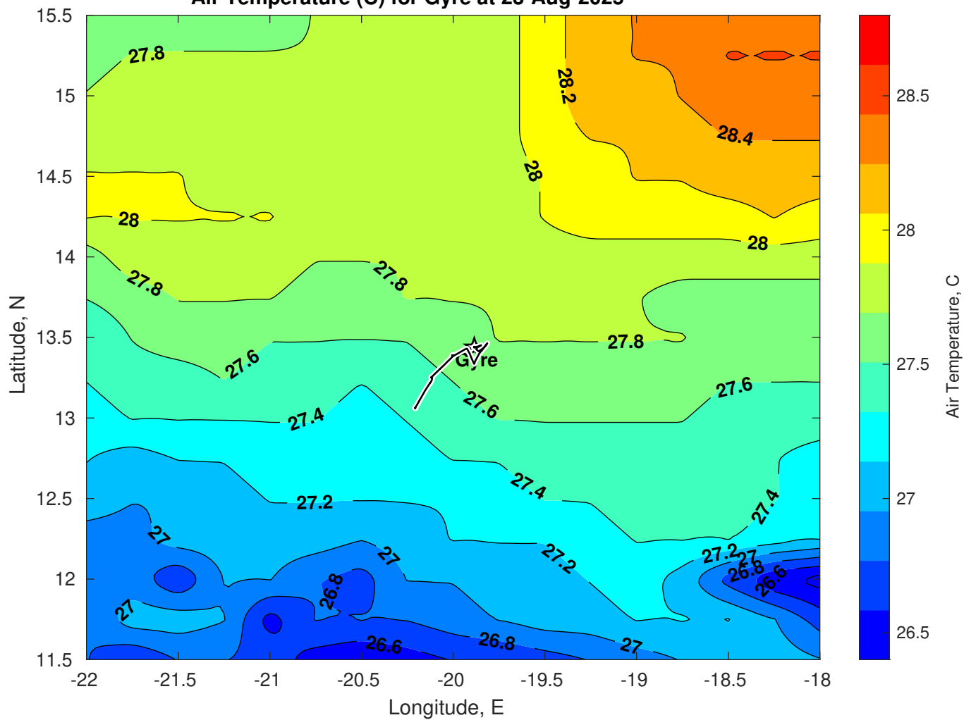
Air Temperature (C) for Gyre at 23-Aug-2025
