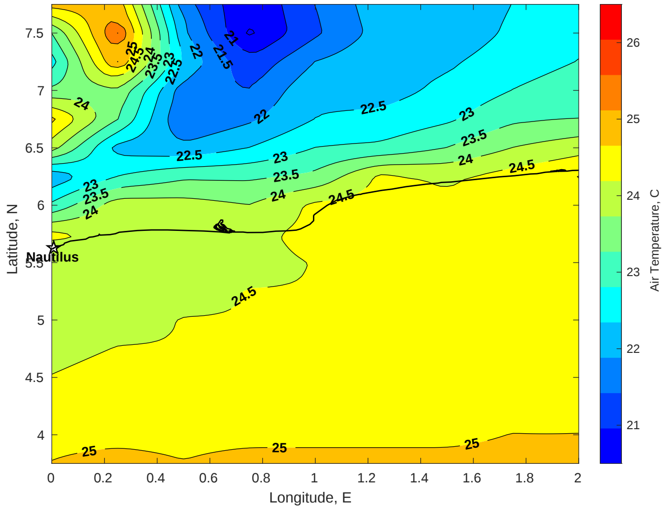
Air Temperature (C) for Nautilus at 23-Aug-2025
