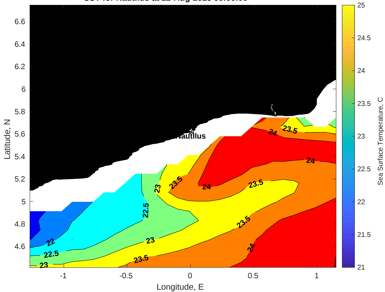
SST for Nautilus at 22-Aug-2025 00:00:00
