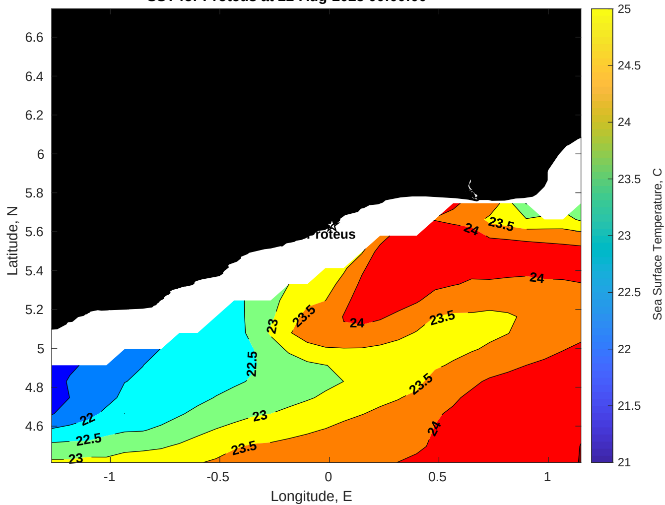
SST for Proteus at 22-Aug-2025 00:00:00
