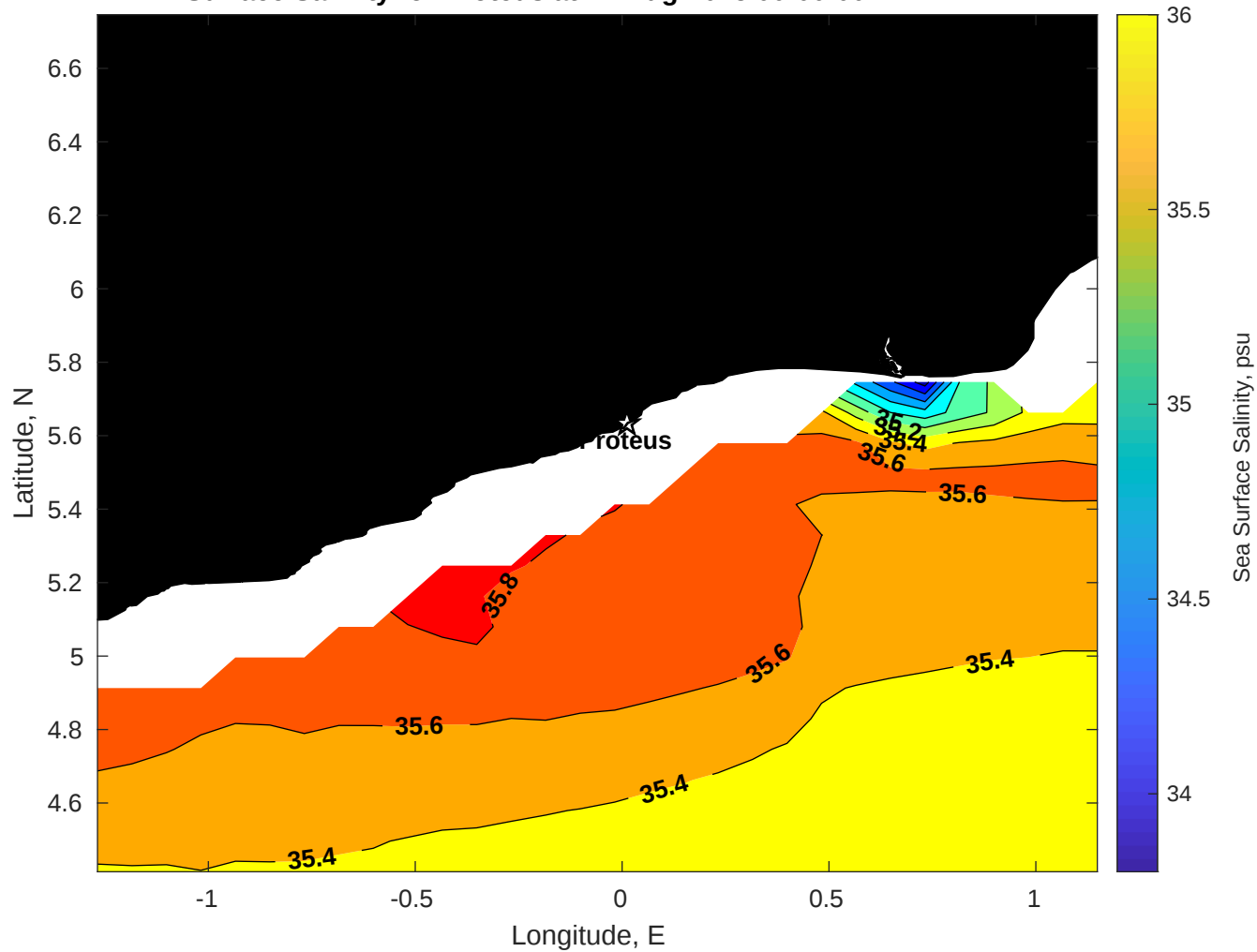
Surface Salinity for Proteus at 22-Aug-2025 00:00:00
