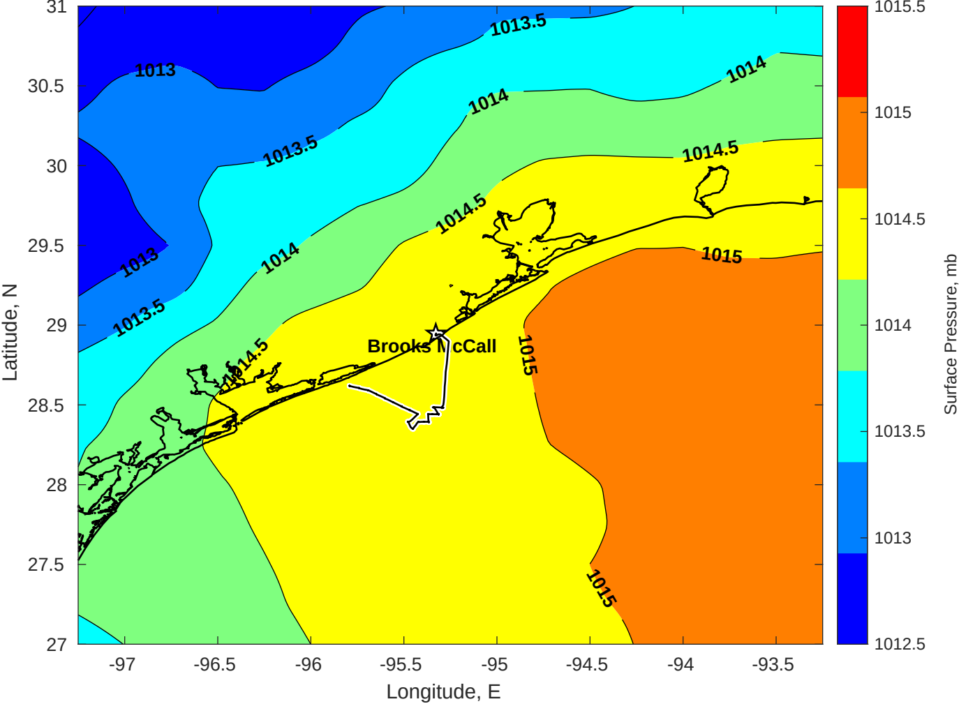
Surface Pressure (mb) for Brooks McCall at 26-Aug-2025 00:00:00
