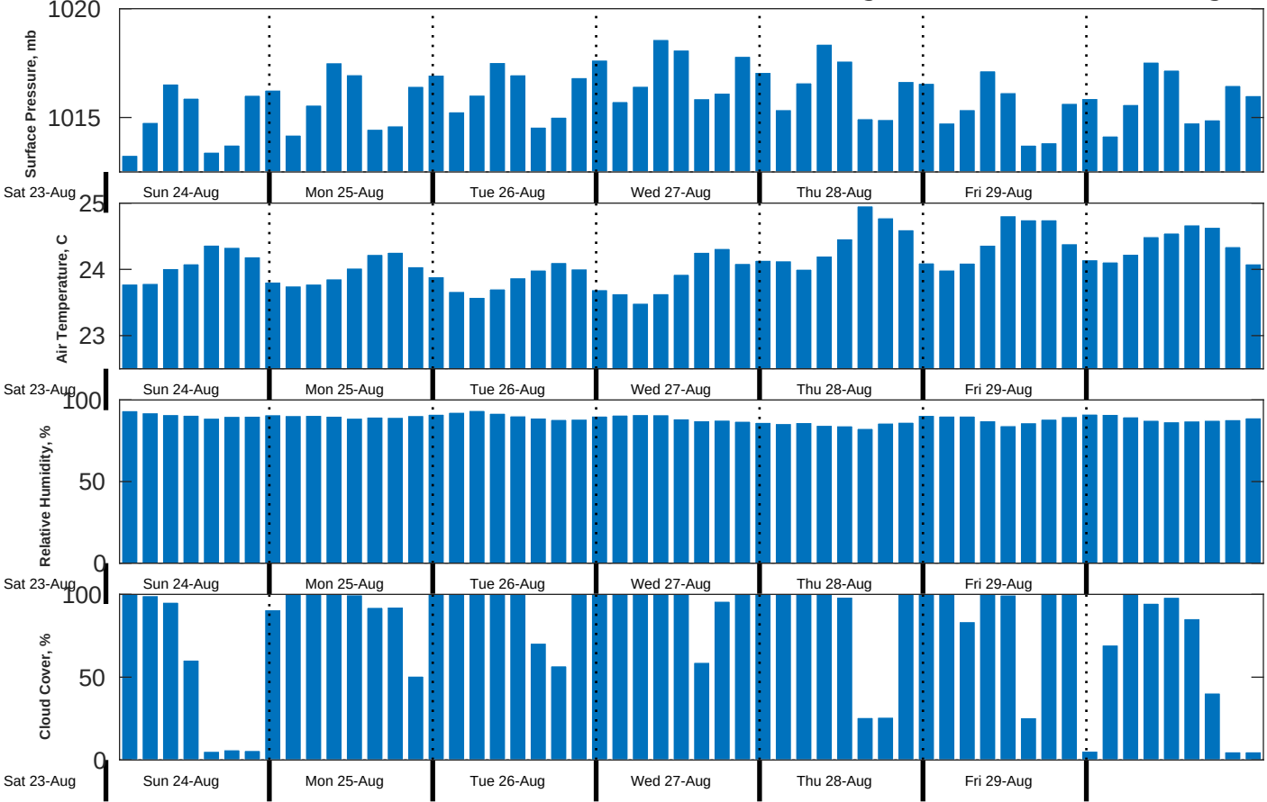
Met Forecast for CSA (ONHYM) PPL EBS - Cote d'Ivoire from 24-Aug-2025 00:00:00 to 31-Aug-2025 00:00:00
