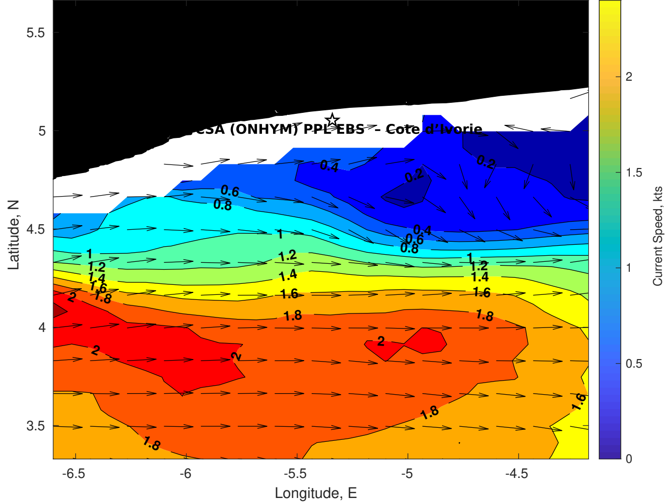
Surface Currents for CSA (ONHYM) PPL EBS - Cote d'Ivoire at 23-Aug-2025 00:00:00
