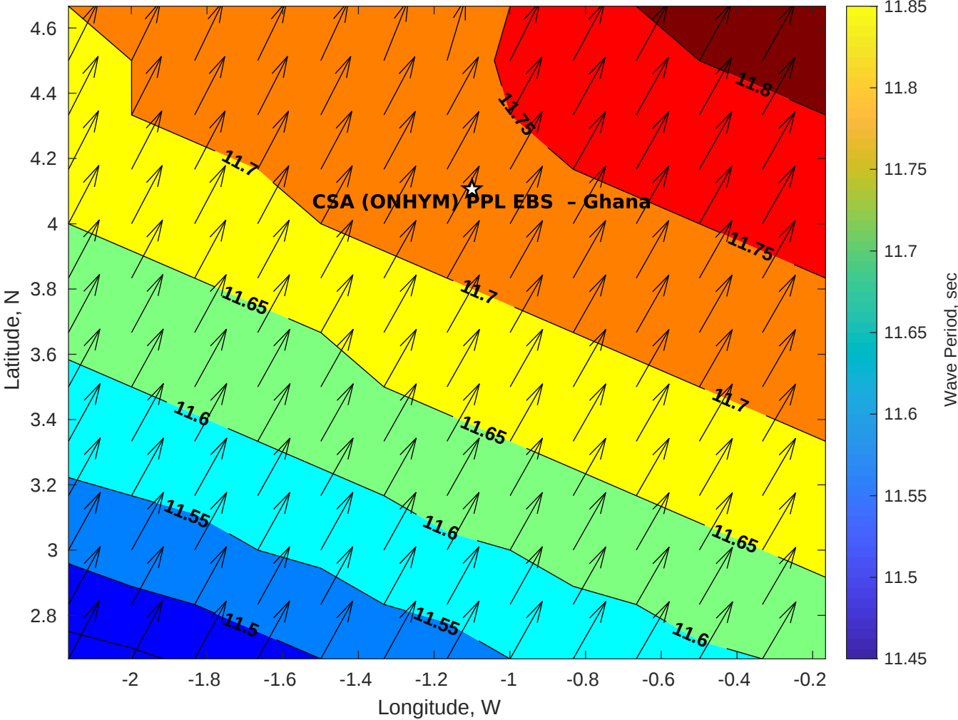
Wave Period (sec) for CSA (ONHYM) PPL EBS - Ghana at 24-Aug-2025 09:00:00
