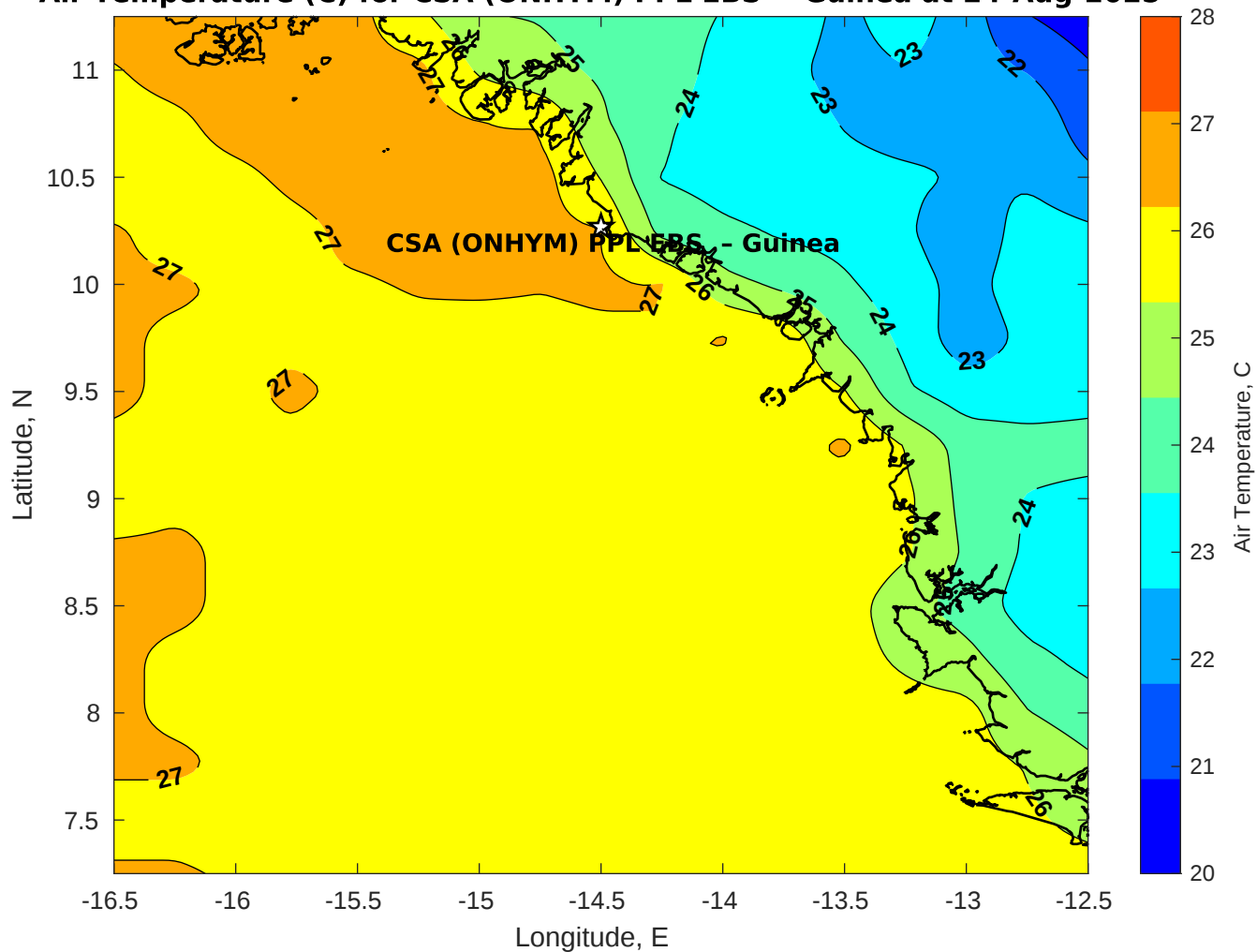
Air Temperature (C) for CSA (ONHYM) PPL EBS - Guinea at 24-Aug-2025
