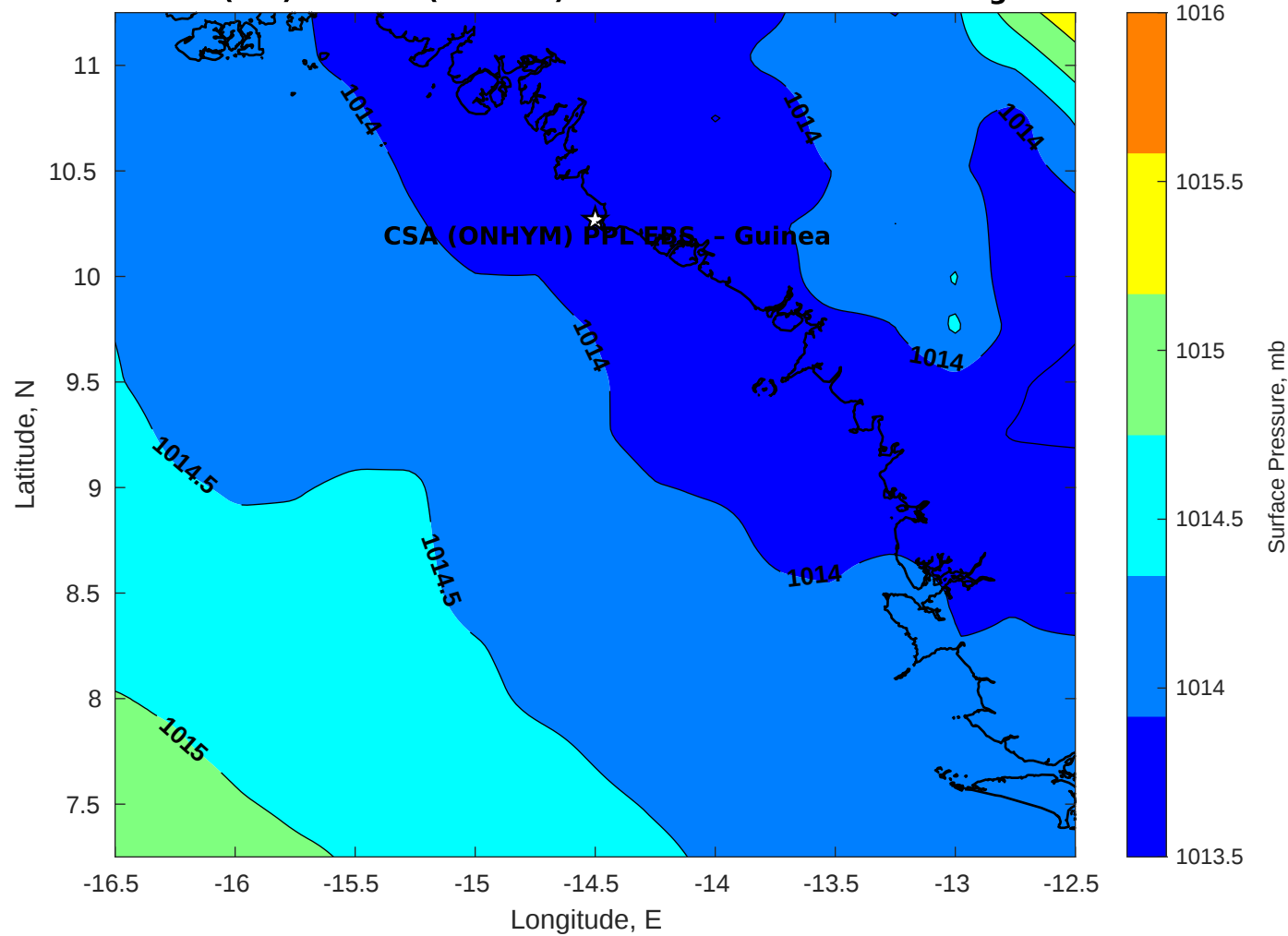
Surface Pressure (mb) for CSA (ONHYM) PPL EBS - Guinea at 24-Aug-2025 00:00:00
