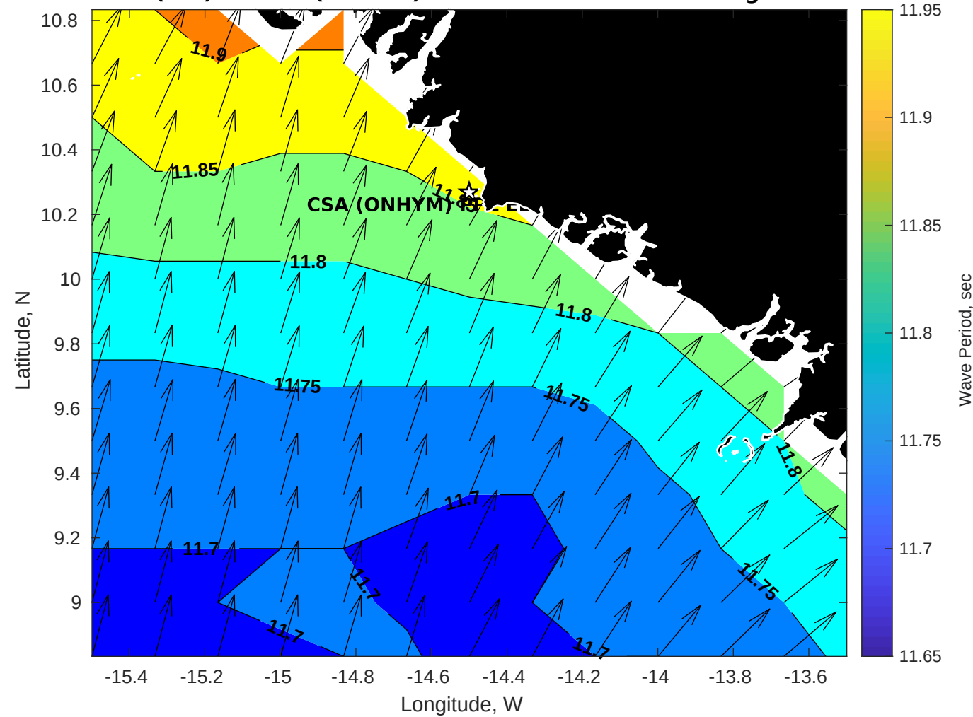
Wave Period (sec) for CSA (ONHYM) PPL EBS - Guinea at 24-Aug-2025 09:00:00
