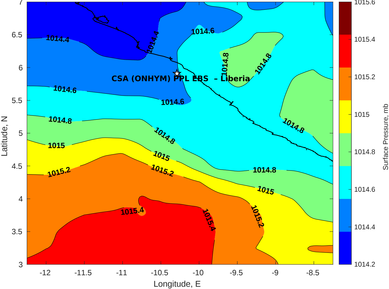
Surface Pressure (mb) for CSA (ONHYM) PPL EBS - Liberia at 24-Aug-2025 00:00:00
