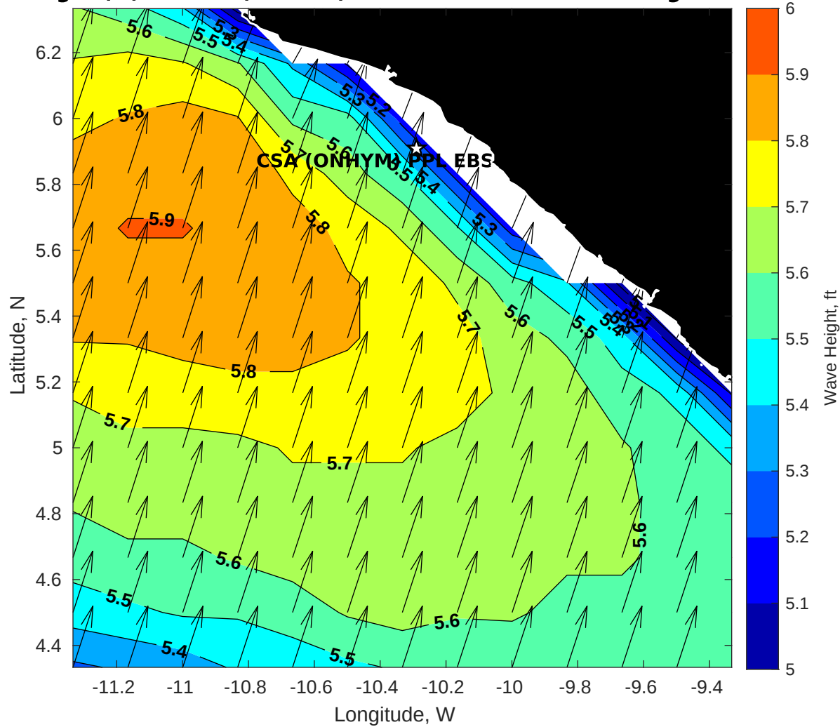
Wave Height (ft) for CSA (ONHYM) PPL EBS - Liberia at 24-Aug-2025 09:00:00
