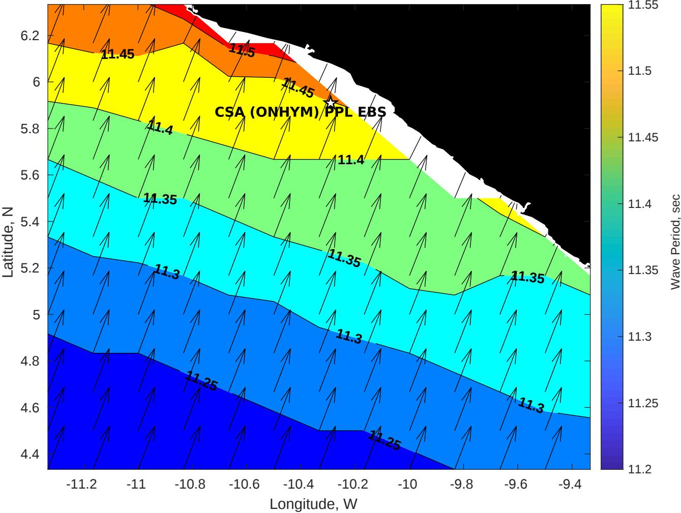
Wave Period (sec) for CSA (ONHYM) PPL EBS - Liberia at 24-Aug-2025 09:00:00
